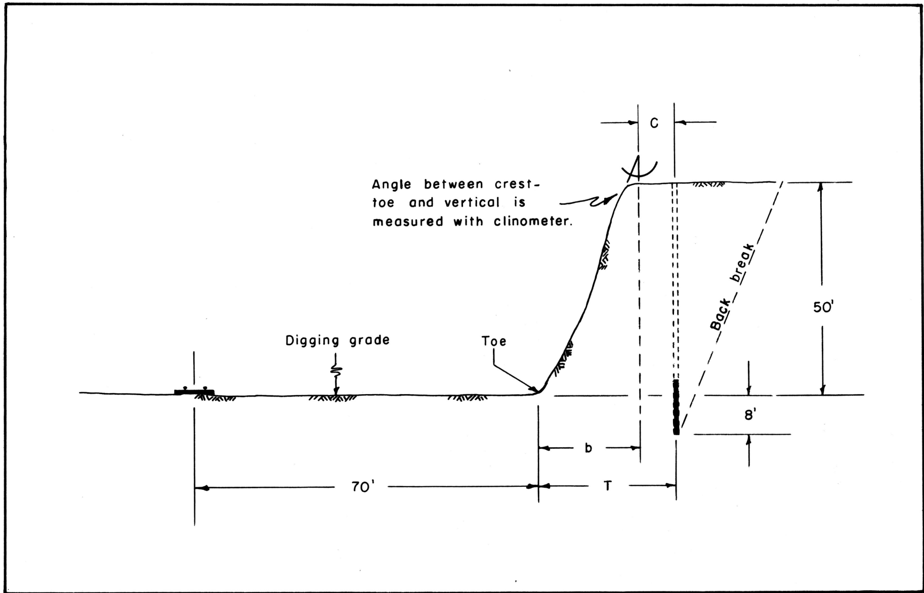
FIGURE-12- ARRANGEMENT OF PRIMARY DRILL HOLE IN BANK - MORENCI MINE
