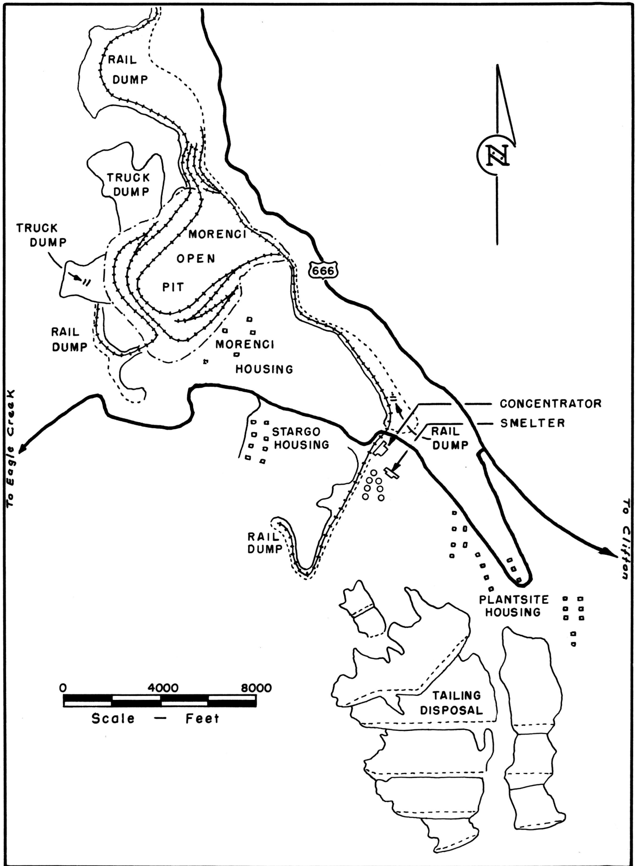
Fig-3-Sketch map, open pit mine and plant Morenci, Arizona
