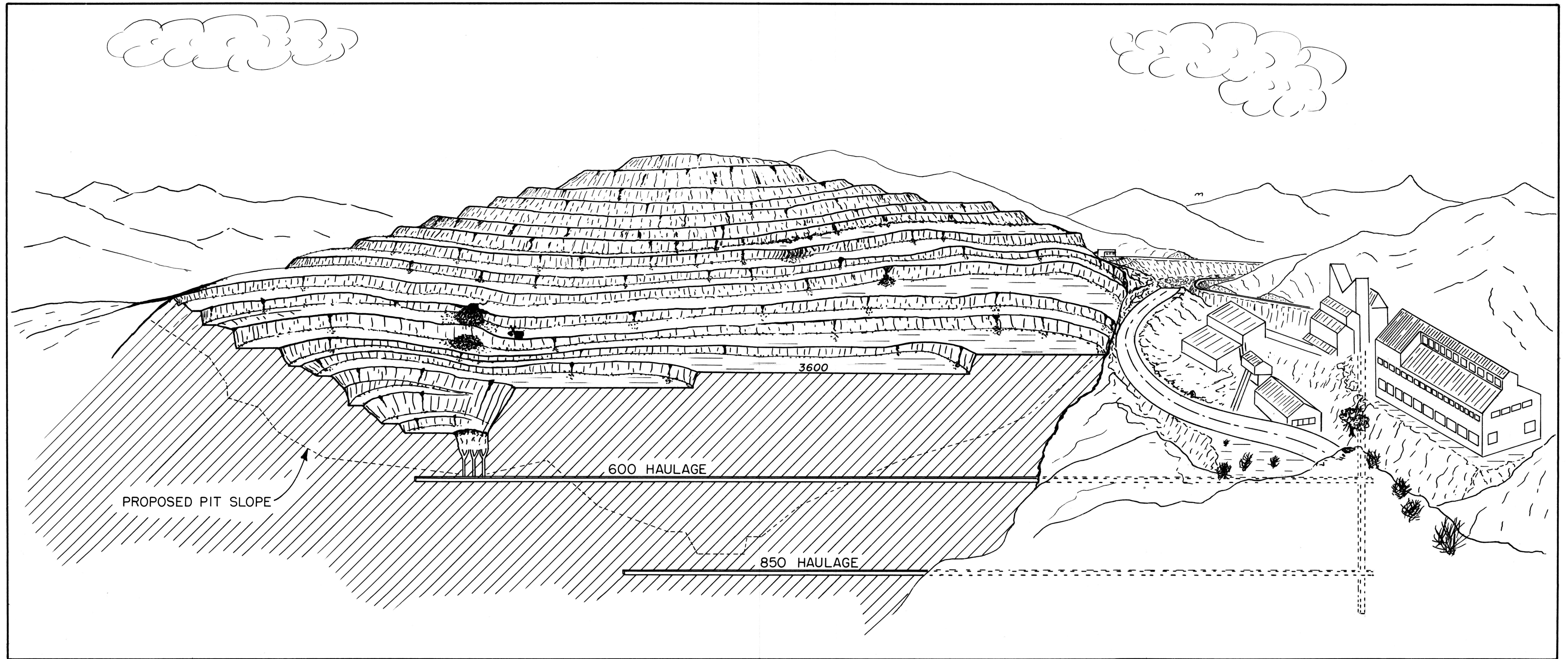
Figure 9.-Profile through Thornton pit and underground haulage system.
