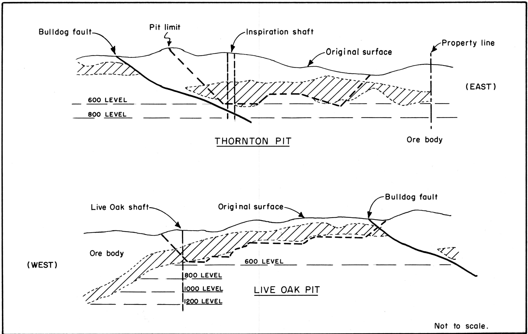
Figure 5.- Section through orebodies and open pits.
