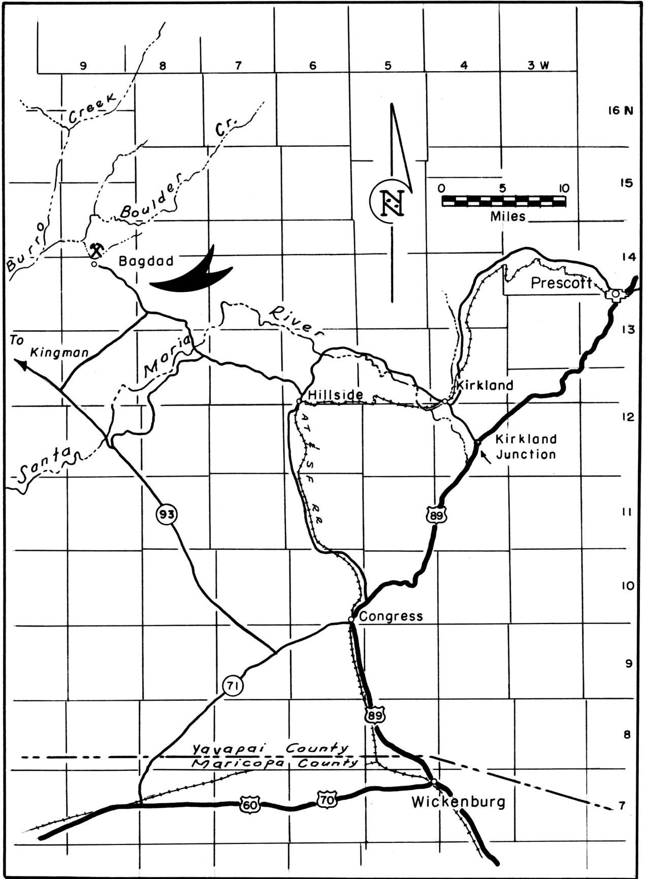
Figure 2. Location map, Bagdad mine Yavapai County, Arizona
