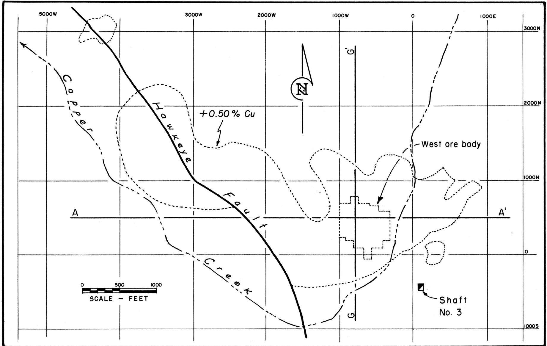
Figure 5. Outline of sulfide ore body.
