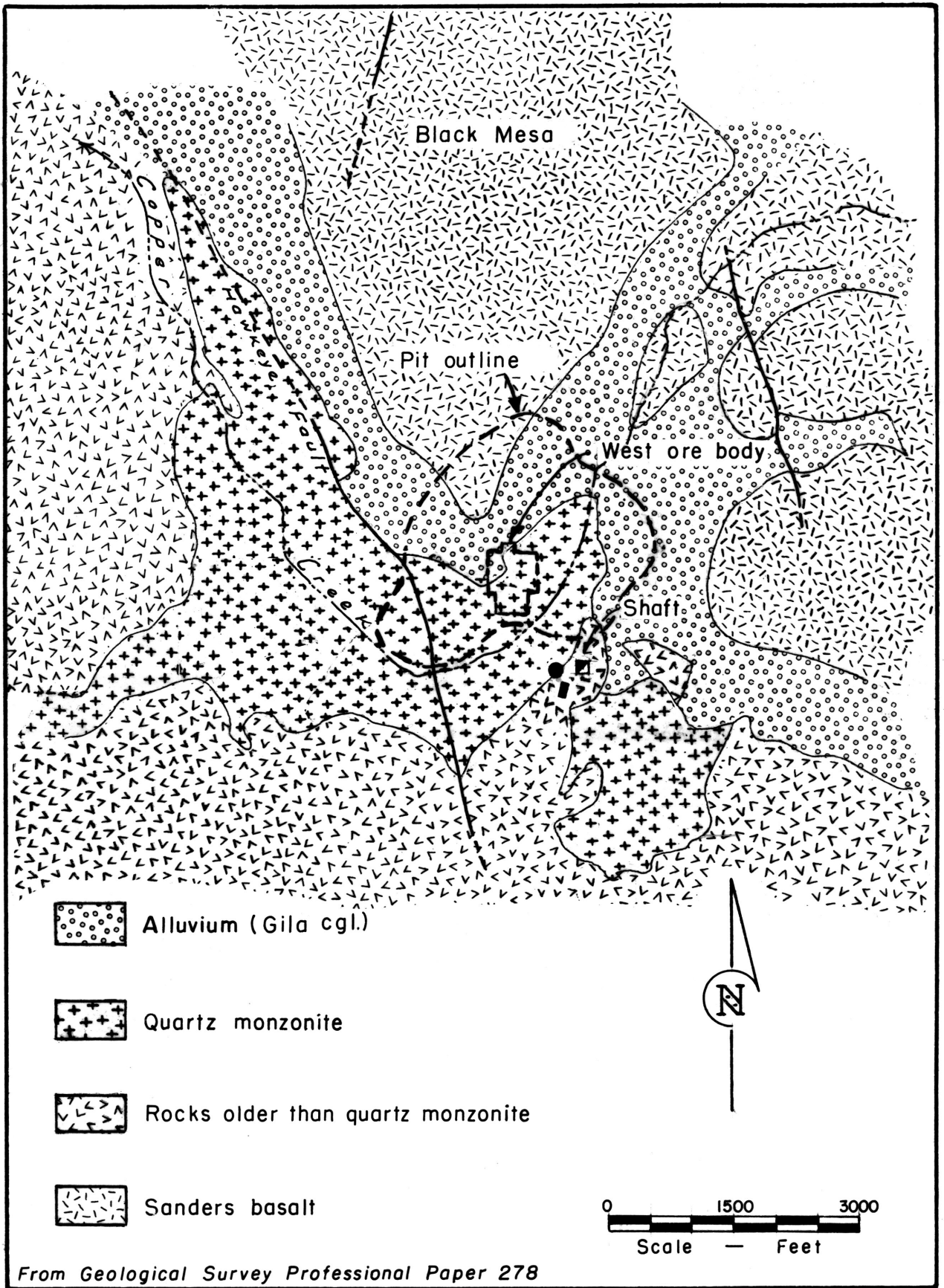
Figure 4. Surface geology, Bagdad mine, Yavapai County.
