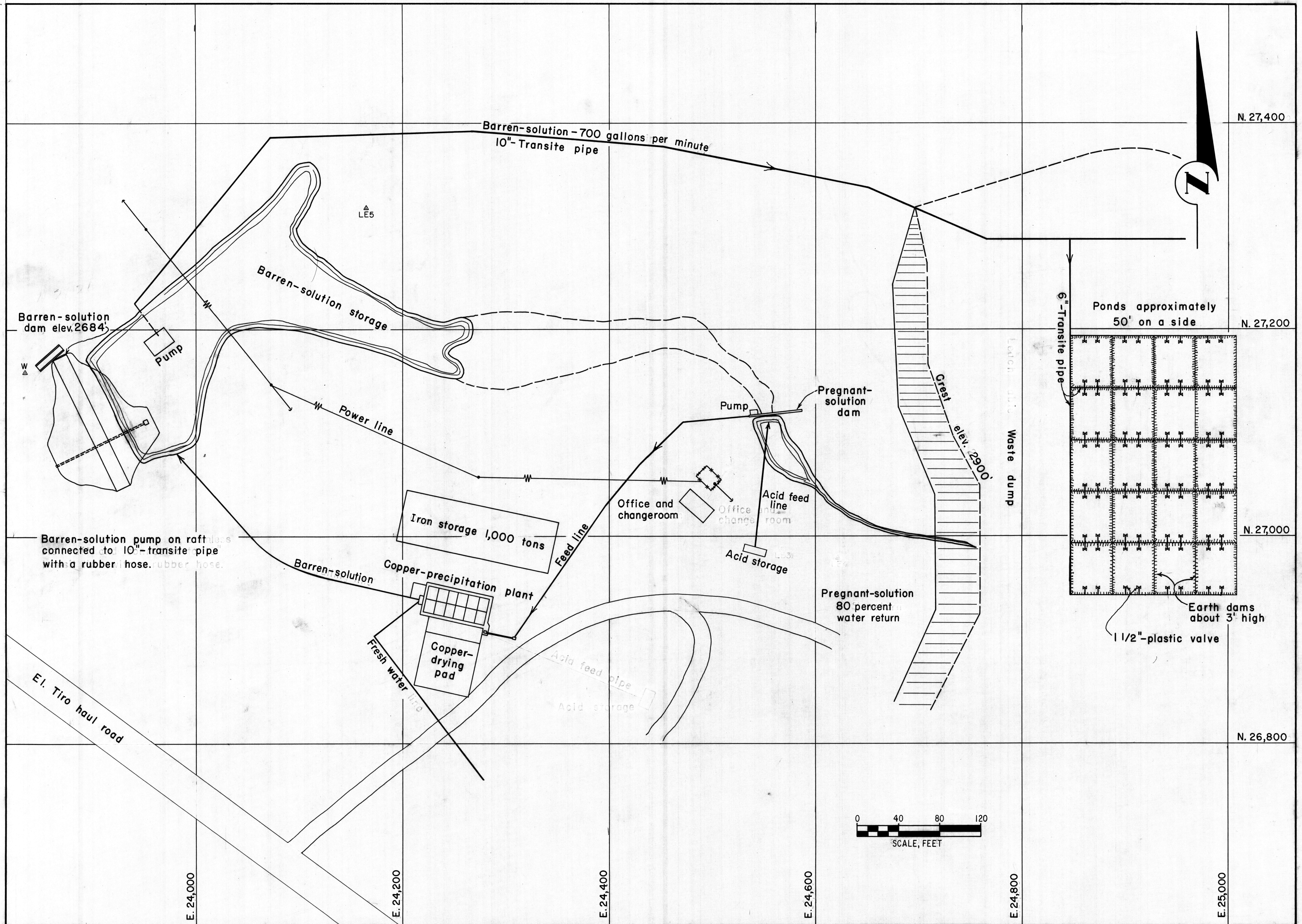
Figure 37.- General Plan of Leaching System
