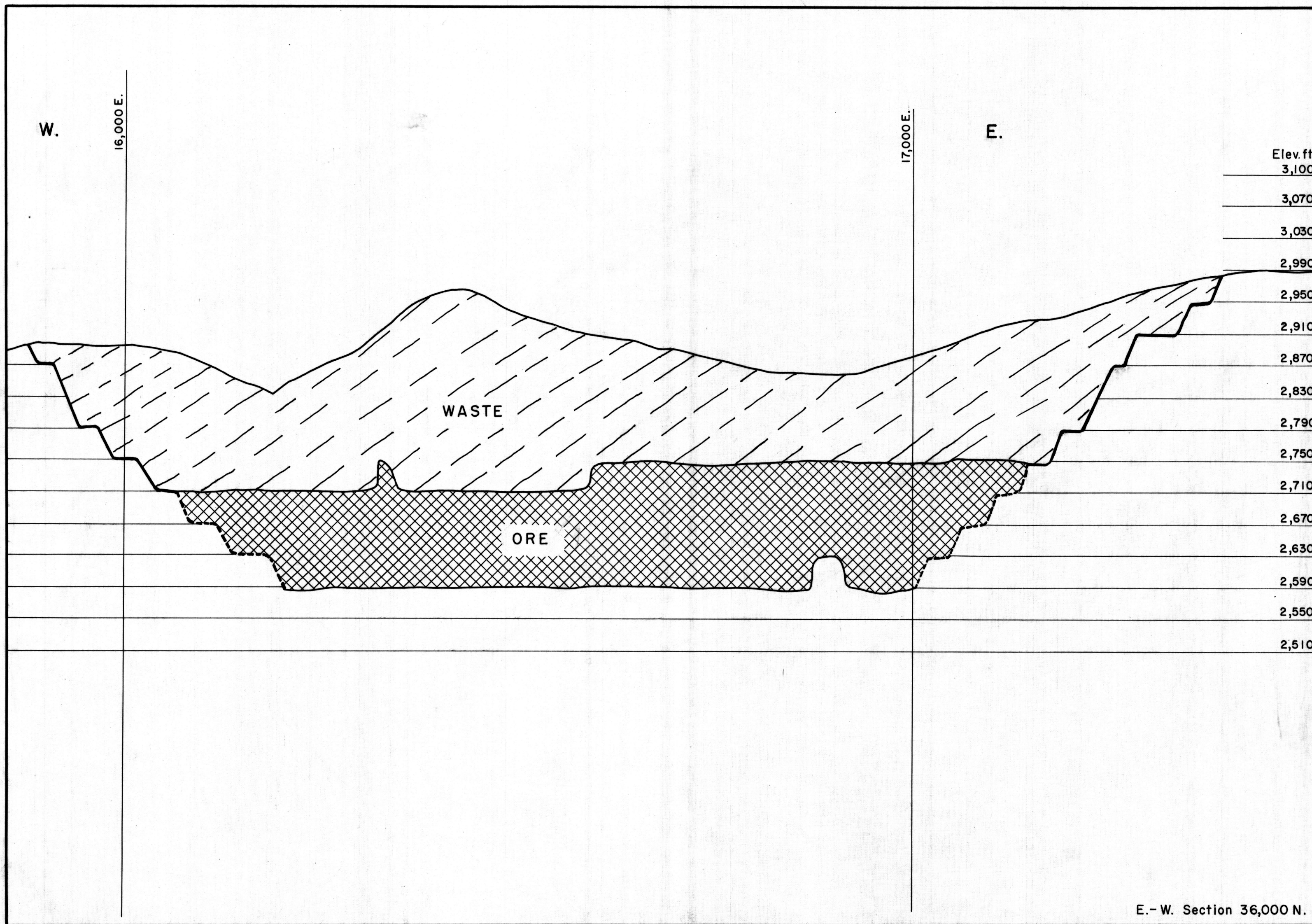
Figure II.- Section Through El Tiro Pit
