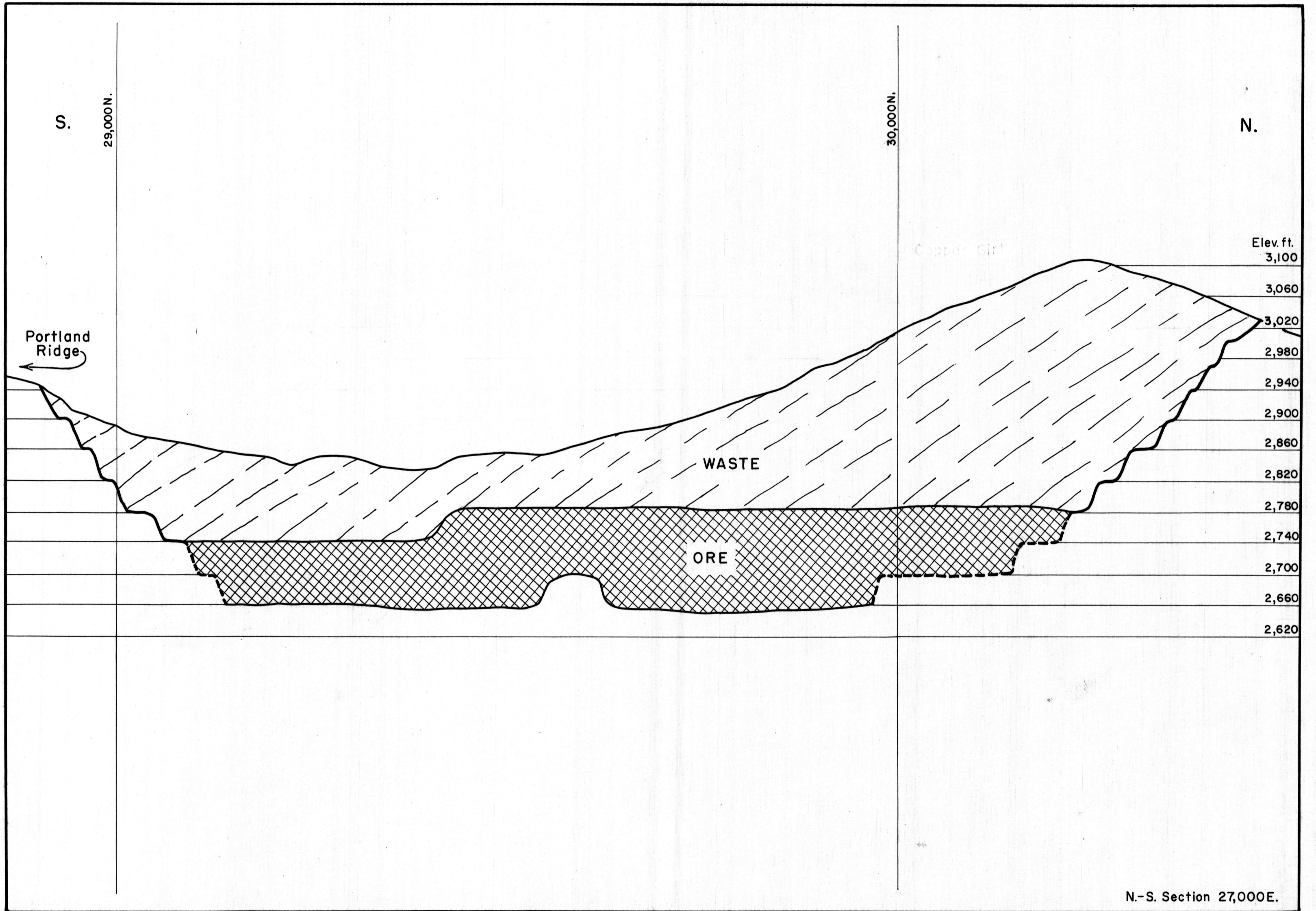
Figure 10.- Section Through Oxide Pit
