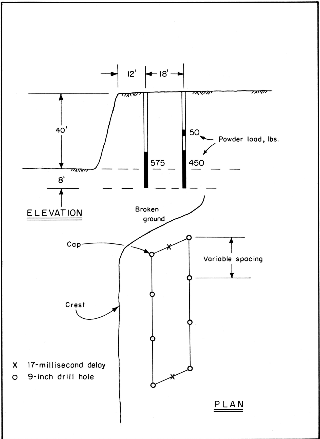
Figure 12-Burden shot.
