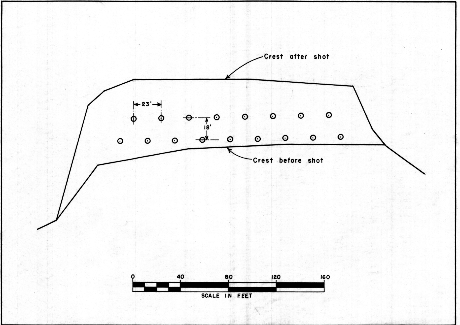
Figure II.- Plan of Typical Burden Shot
