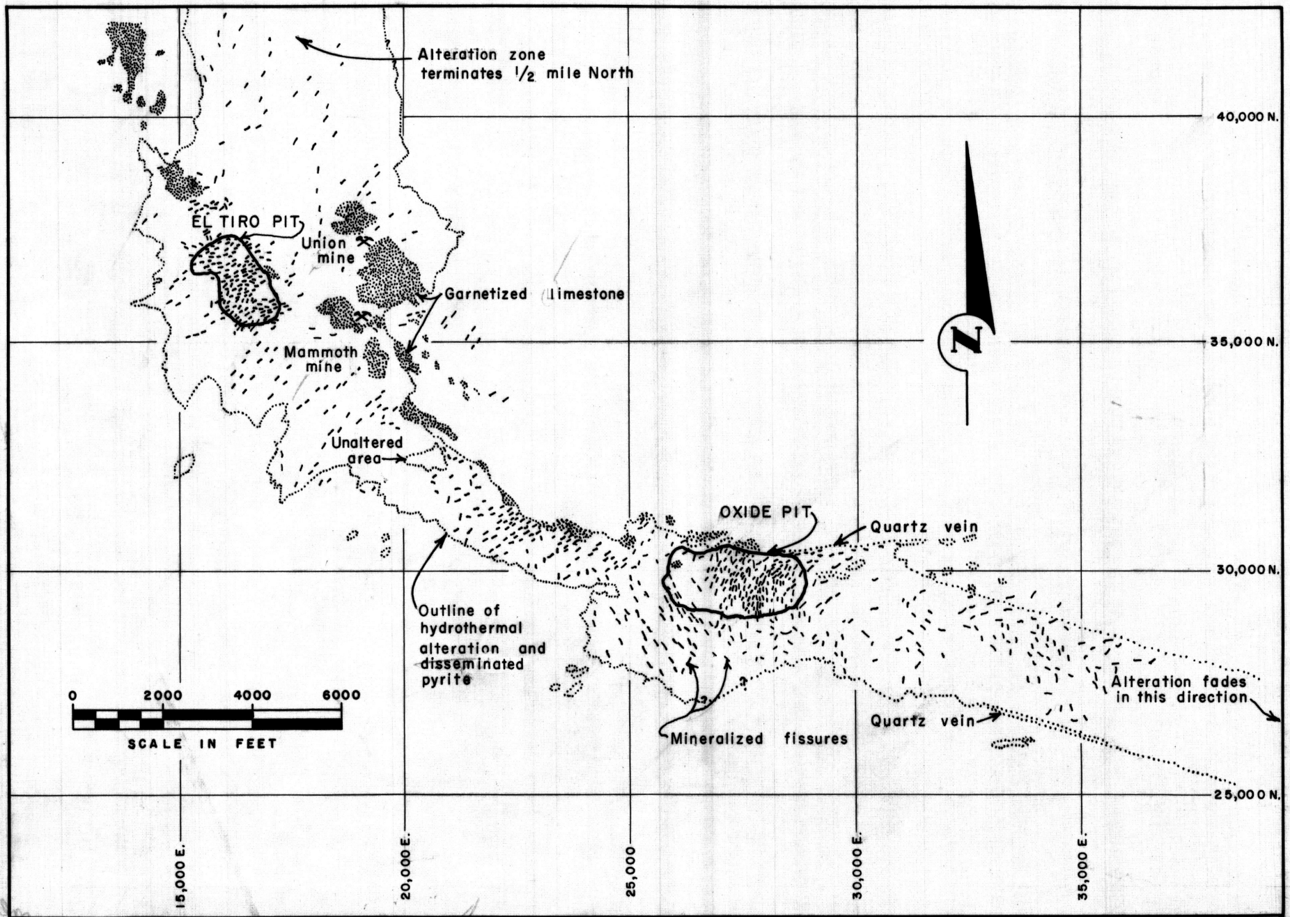
Figure 4.- Zone of Hydrothermal Alteration
