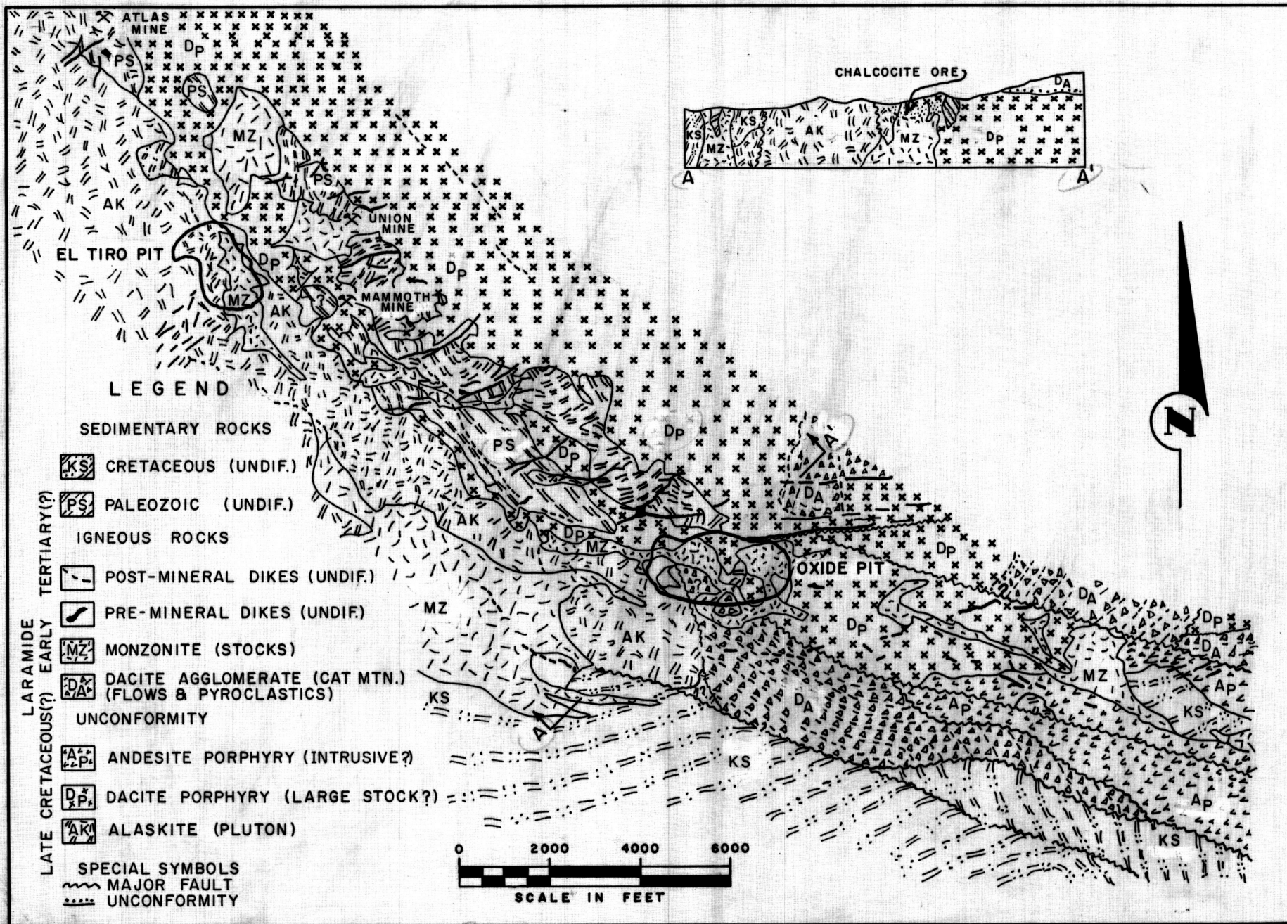
Figure 3.- Geology of Silver Bell District
