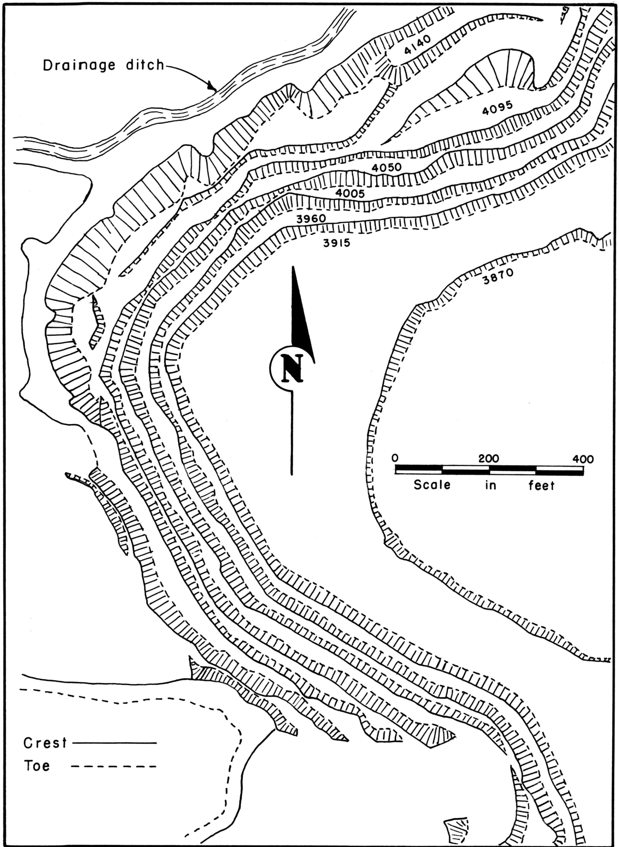
Figure 29. Plan of banks trimmed to trial final slope, Copper Cities mine
