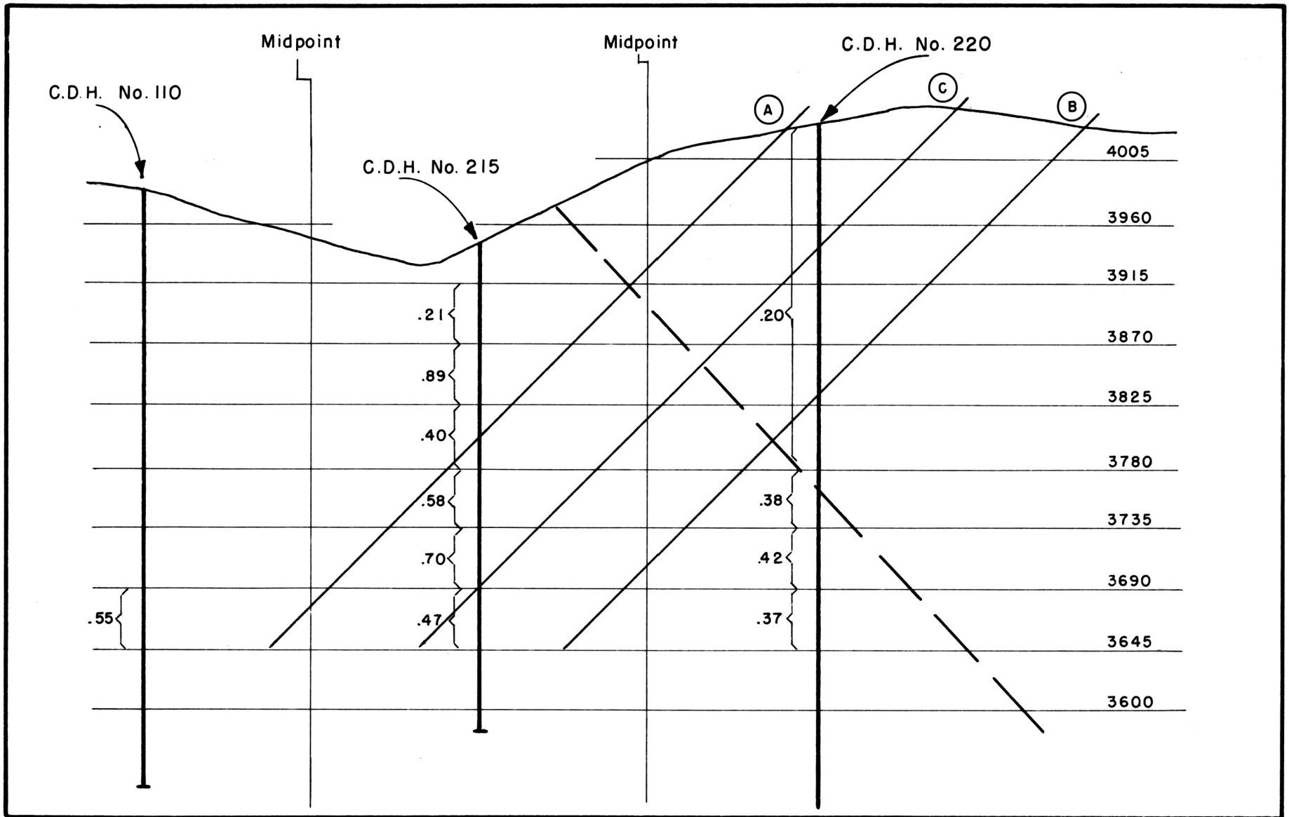
Figure 4. Portion of section N 3500 illustrating investigation of slope line
