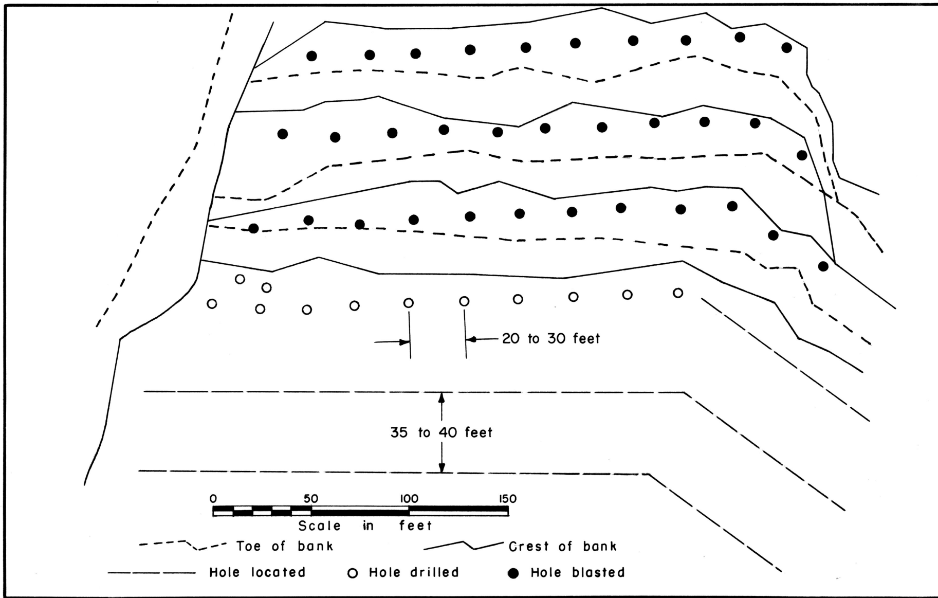
Figure 9. Arrangement of located, drilled & blasted holes
