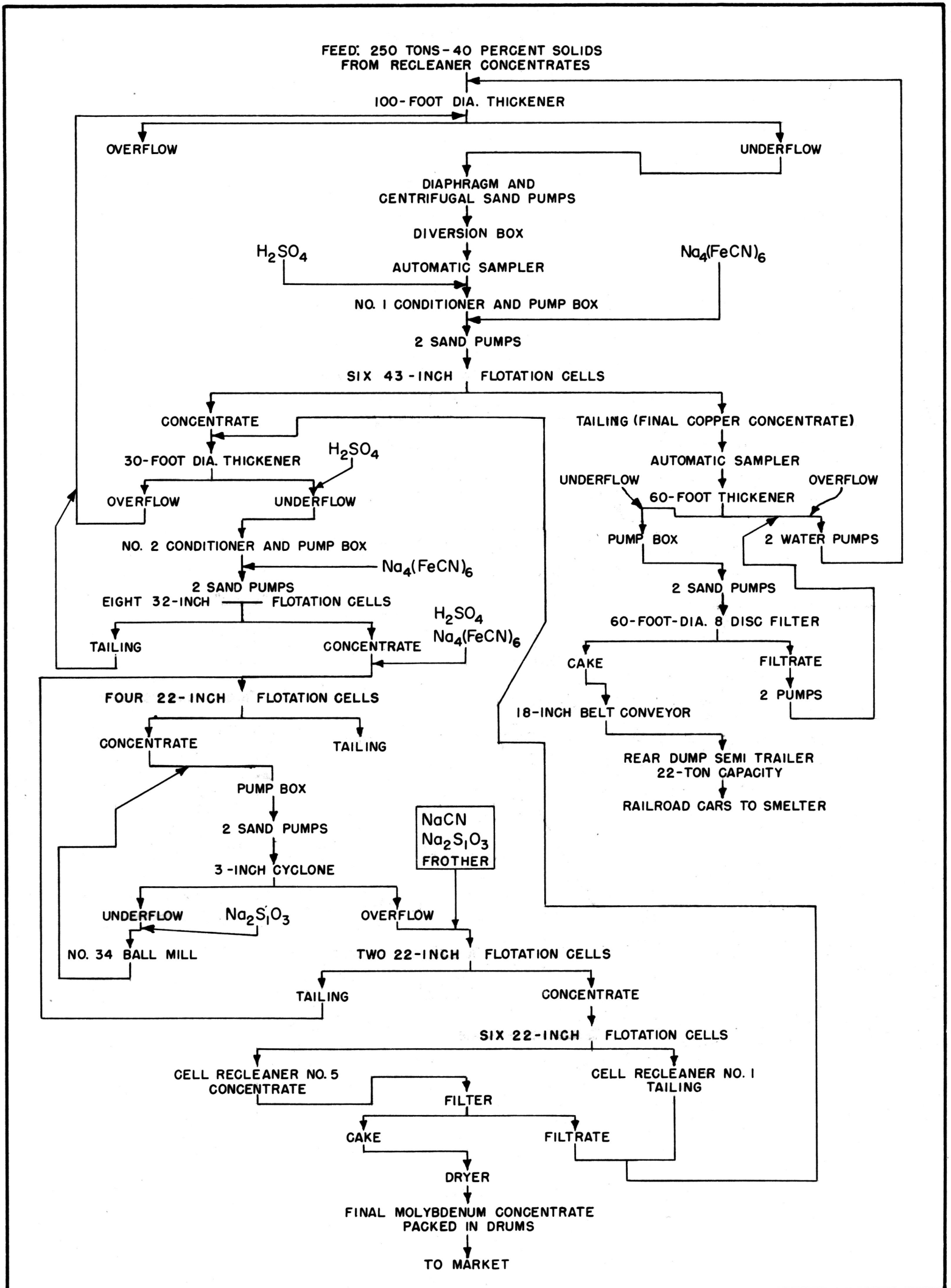
Figure 33.-Flowsheet of molybdenum section.
