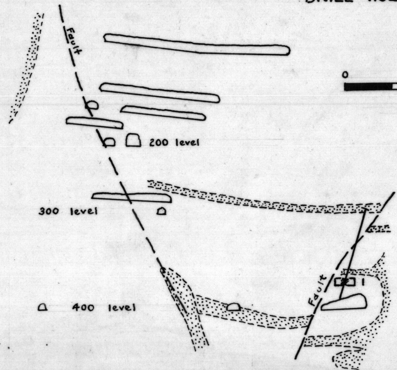
FIG. 28 - SECTIONS THROUGH HOLES DRILLED FROM 400 LEVEL SHOWING ORE BLOCKS.
