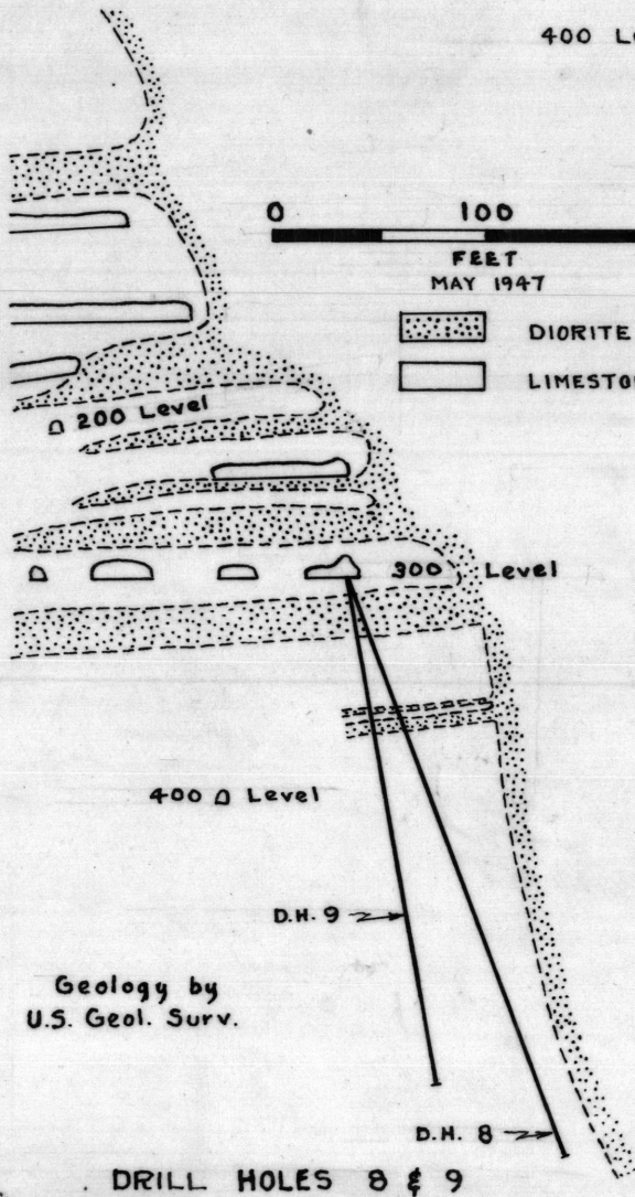
FIG. 27 - SECTIONS THROUGH HOLES DRILLED FROM 300 LEVEL SHOWING ORE BLOCKS.
