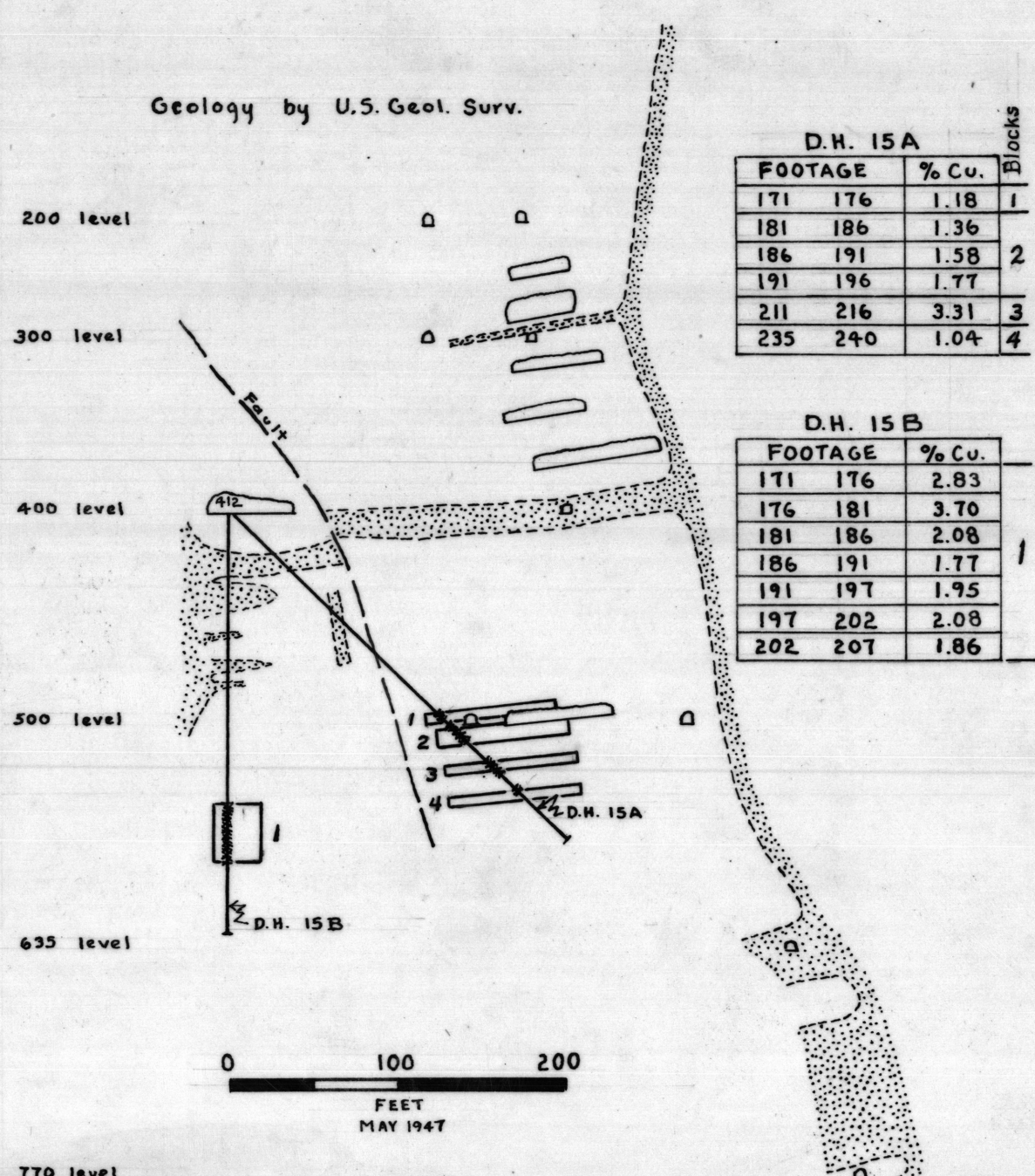
FIG. 25 - SECTION THROUGH HOLES DRILLED FROM 400 LEVEL SHOWING ORE BLOCKS.
