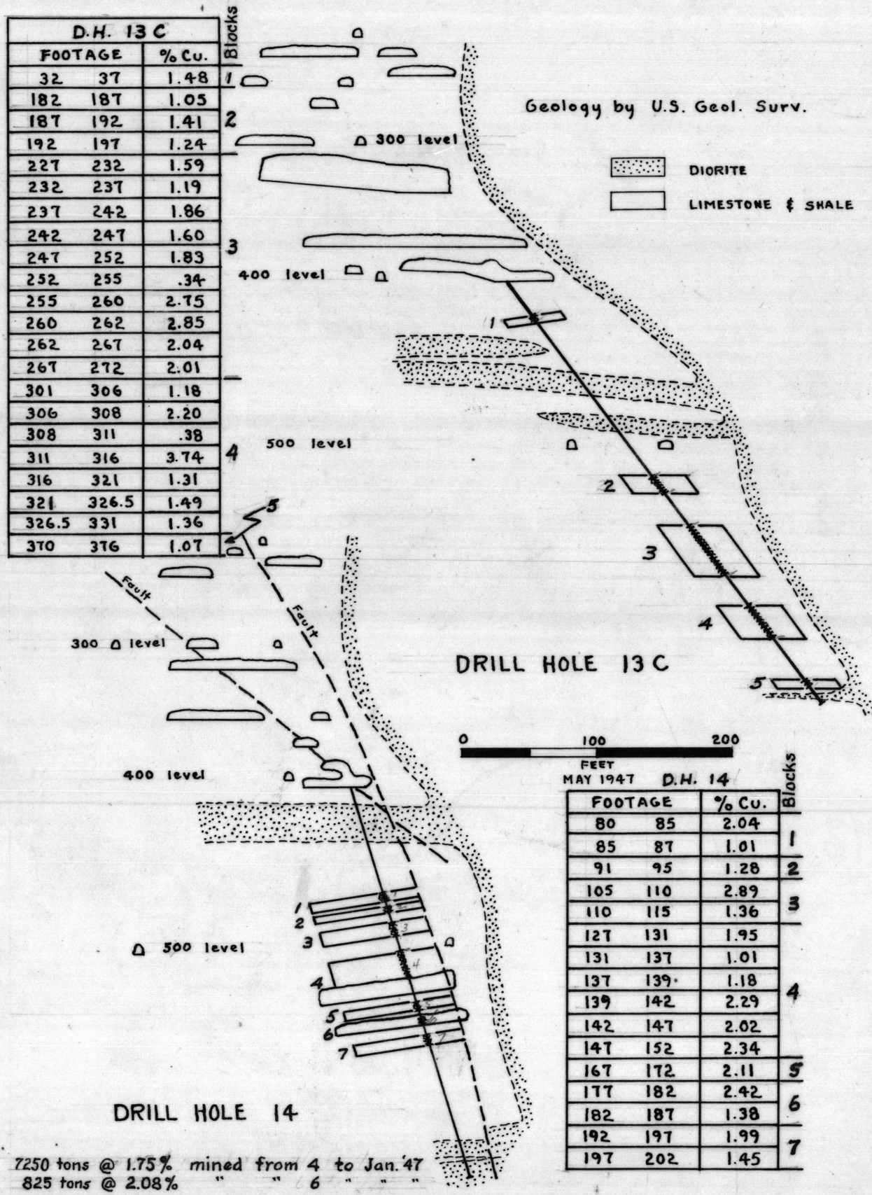
FIG. 24 - SECTIONS THROUGH HOLES DRILLED FROM 400 LEVEL SHOWING ORE BLOCKS.
