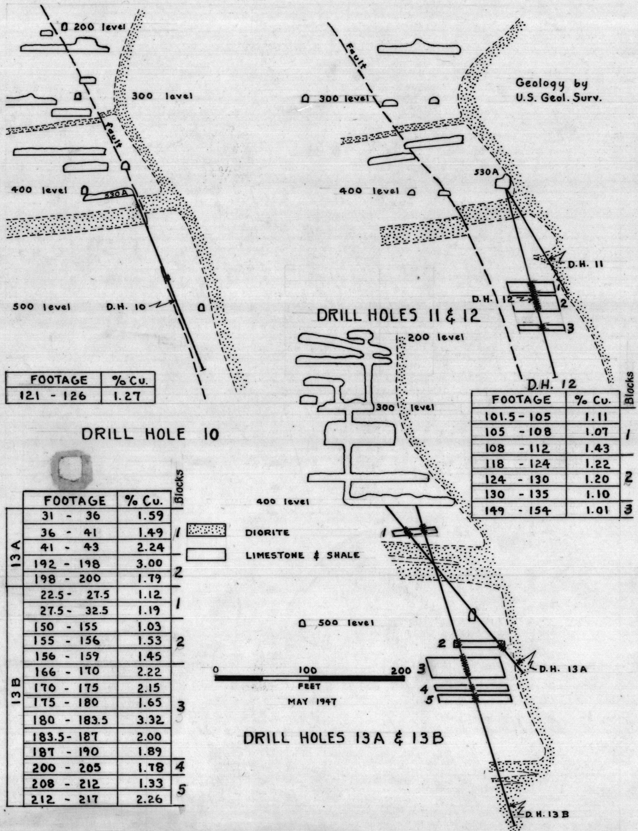
FIG. 23 - SECTIONS THROUGH HOLES DRILLED FROM 400 LEVEL SHOWING ORE BLOCKS.
