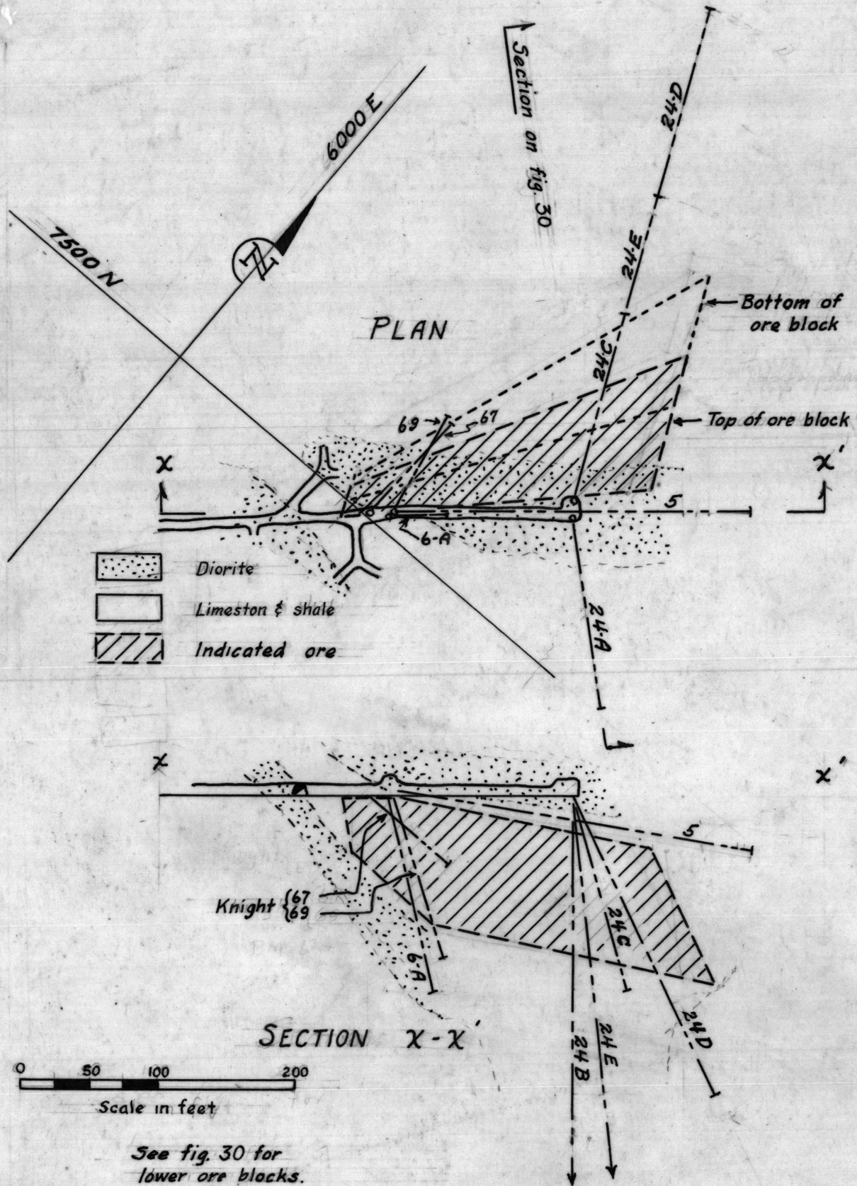
FIG. 31-PLAN & SECTION, NORTH END 770 LEVEL, SHOWING UPPER ORE BLOCKS.
