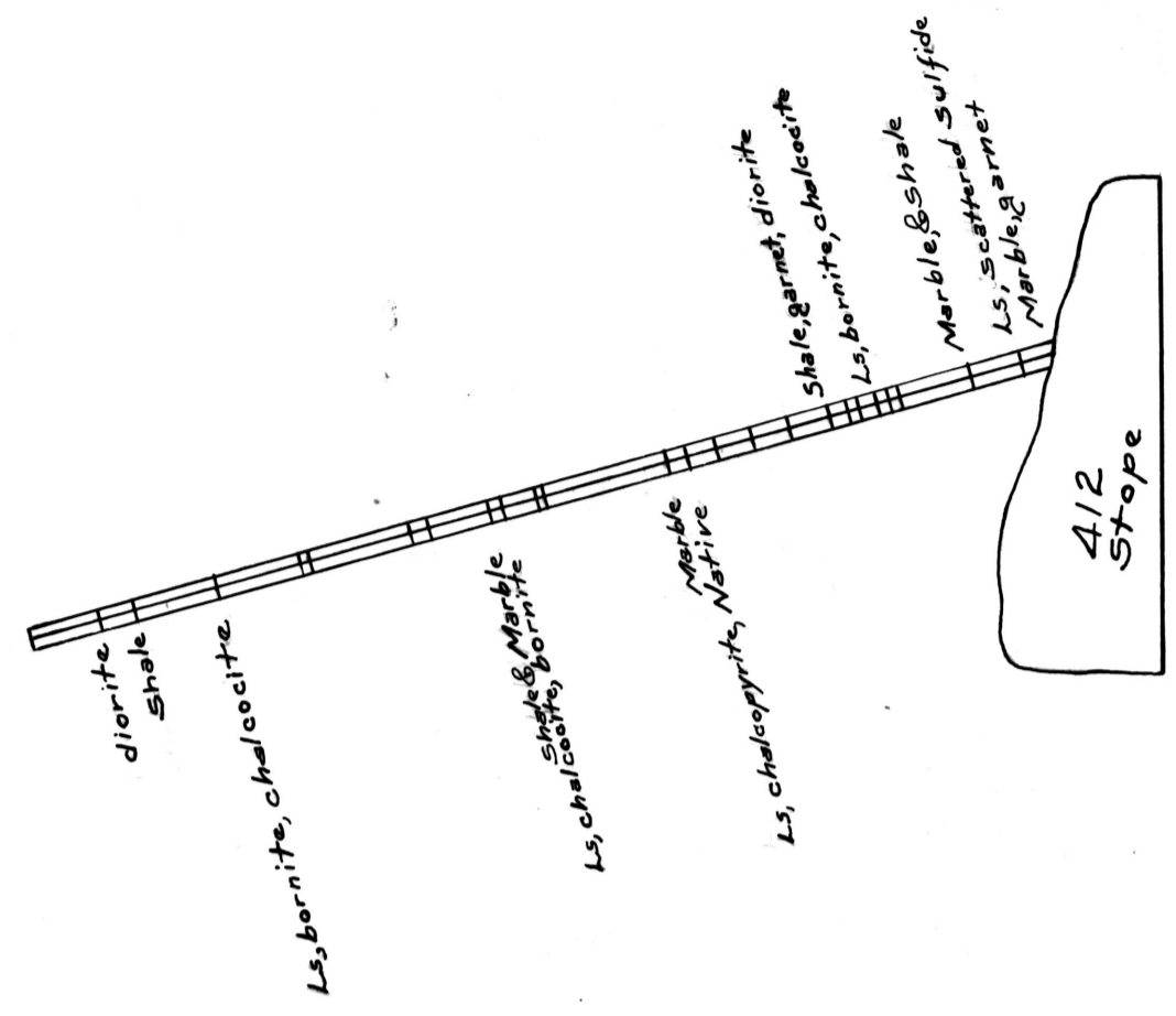
Section Thru D.D.H. 20 Looking West
