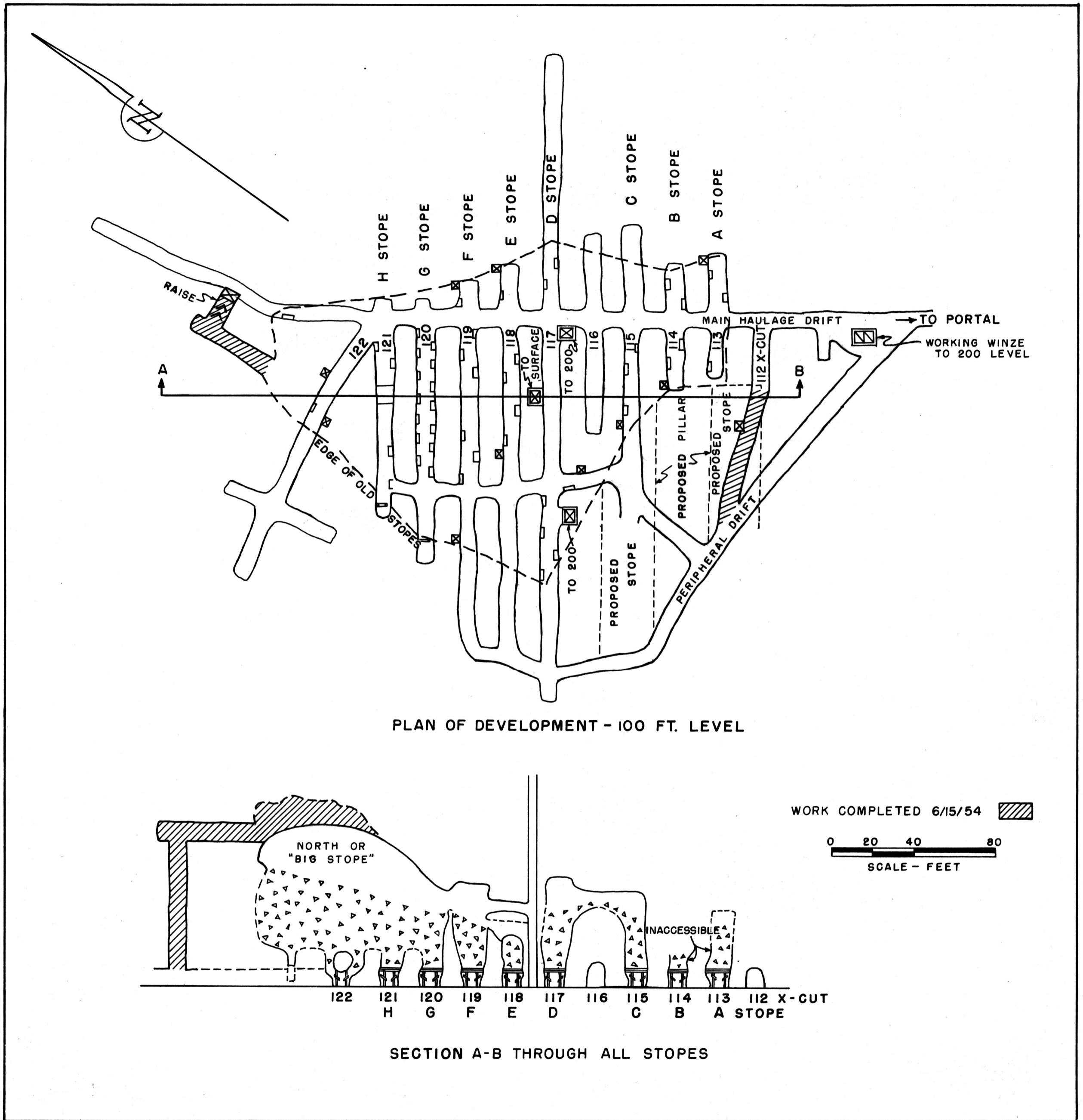
FIGURE I. - 100 FOOT LEVEL - OLD RELIABLE COPPER MINE - PINAL COUNTY, ARIZONA COPPER CREEK CONSOLIDATED MINING COMPANY DMP-84
