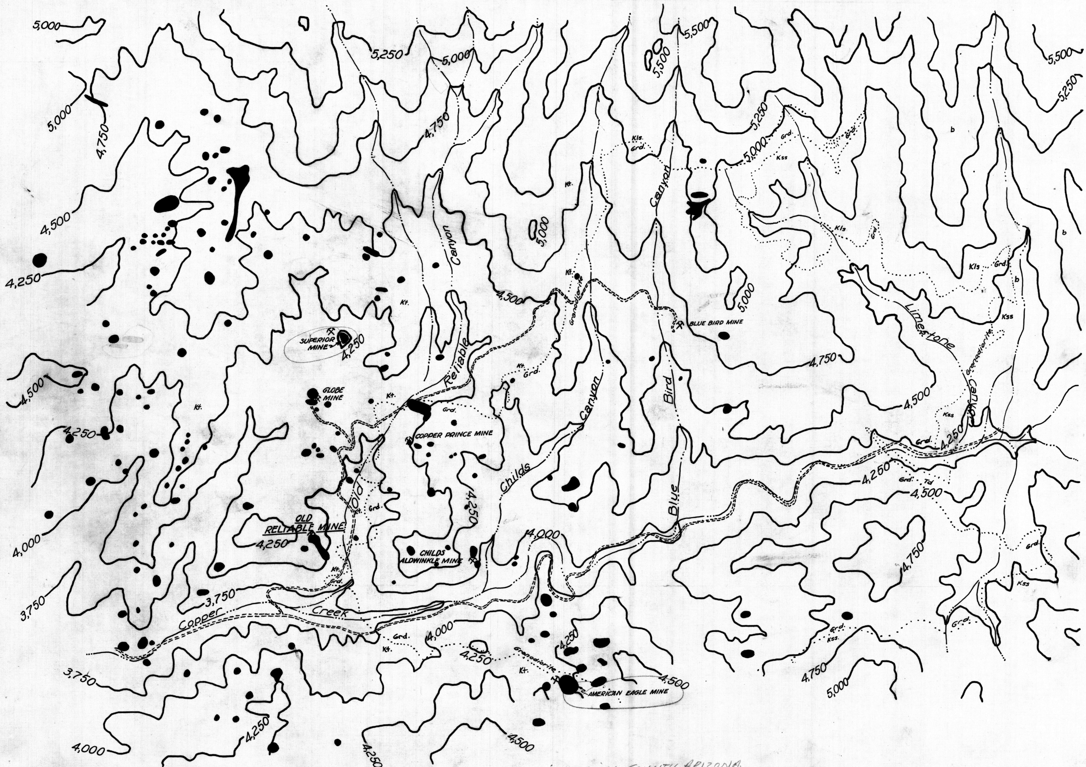
FIG. 11, MAP SHOWING COPPER CREEK AREA BRECCIA ORE PIPES (Geology by Truman H. Kuhn)
