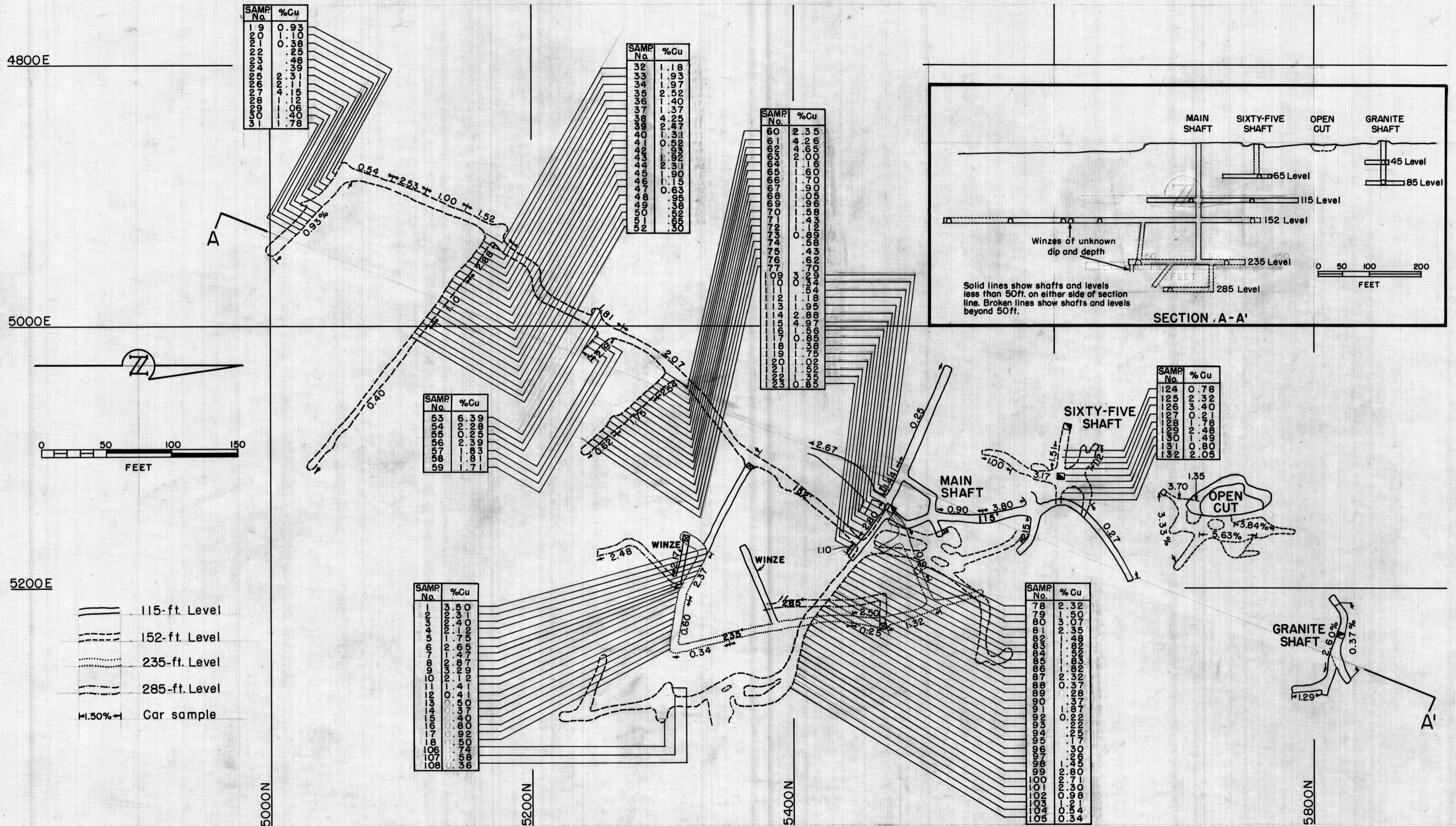
Figure 4 - Assay map, Lake Shore Copper Deposits, Pinal County, Arizona.
