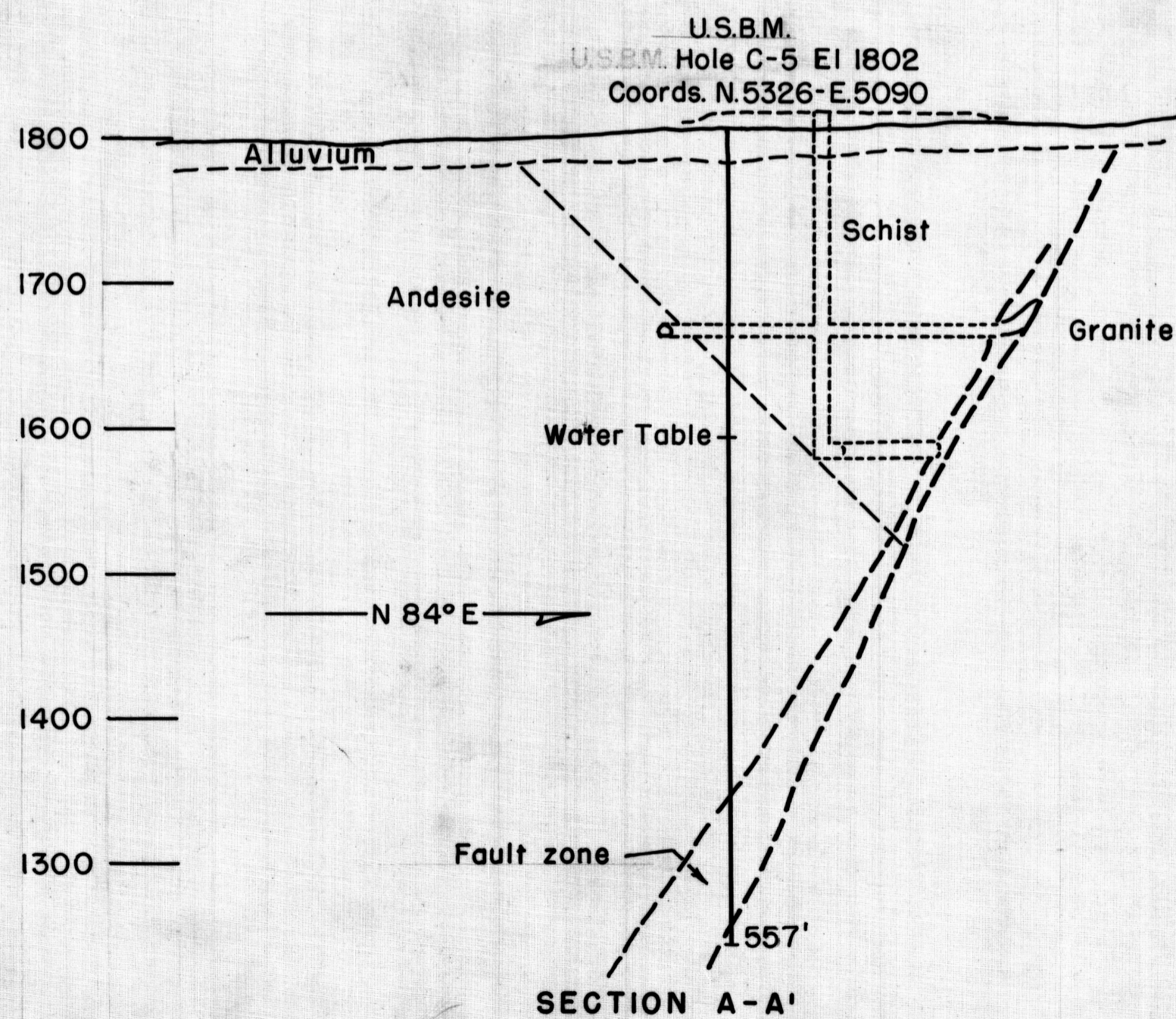
Figure 5 - Geologic sections, Lake Shore Copper Deposits, Pinal County, Arizona.
