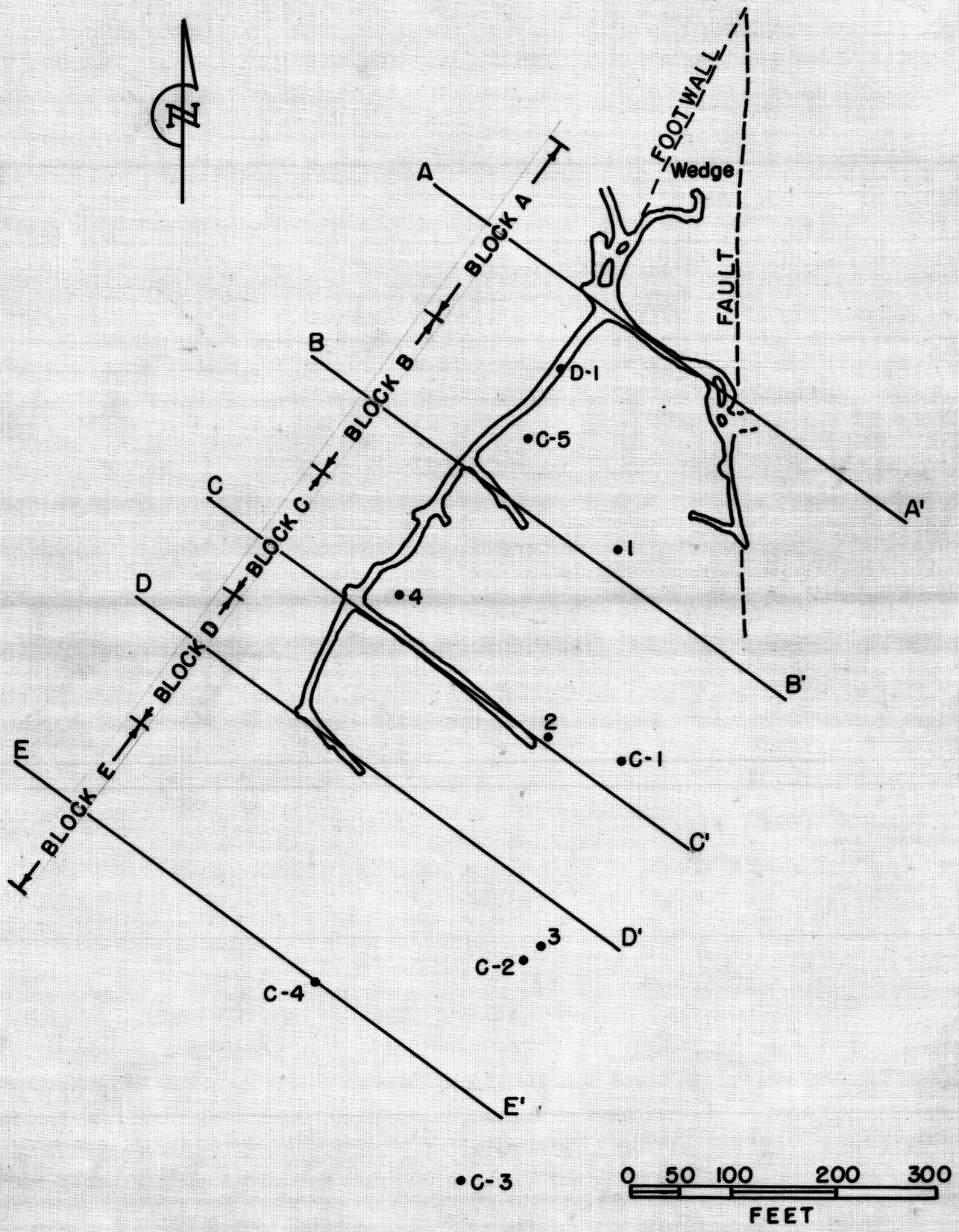
Figure 9- Ore blocks, Lake Shore Copper Deposits, Pinal Co., Ariz.
