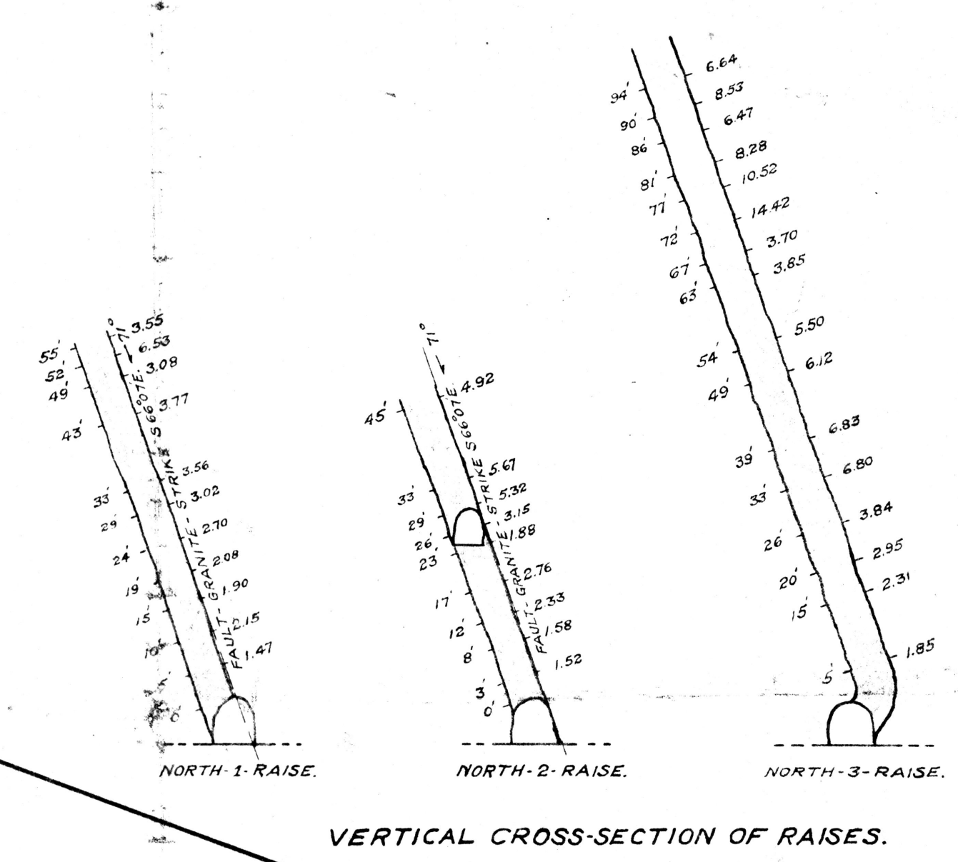
VERTICAL CROSS-SECTION OF RAISES.
