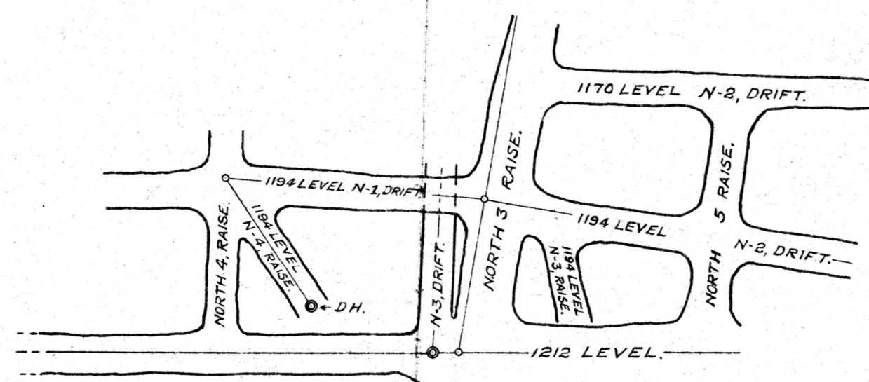
HORIZONTAL PROJECTION.
