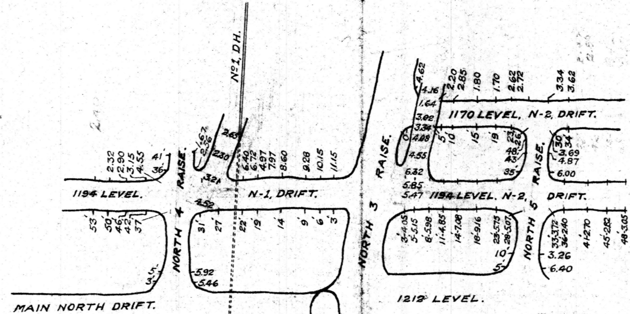
VERTICAL PROJECTION PLANE OF PROJECTION N35°47W.
