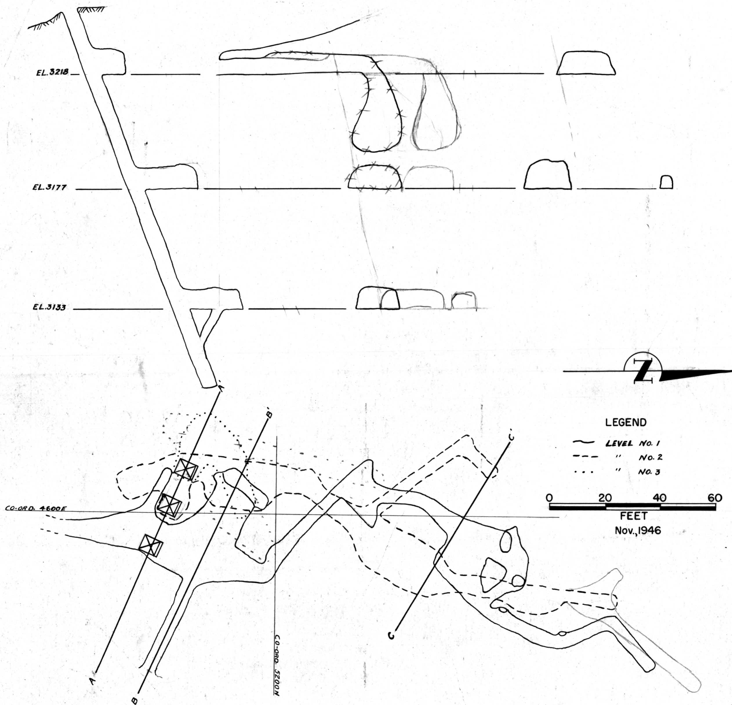
COMPOSITE AND SECTIONS OF UPPER ADIT WORKINGS, ANTLER MINE, MOHAVE COUNTY, ARIZONA
