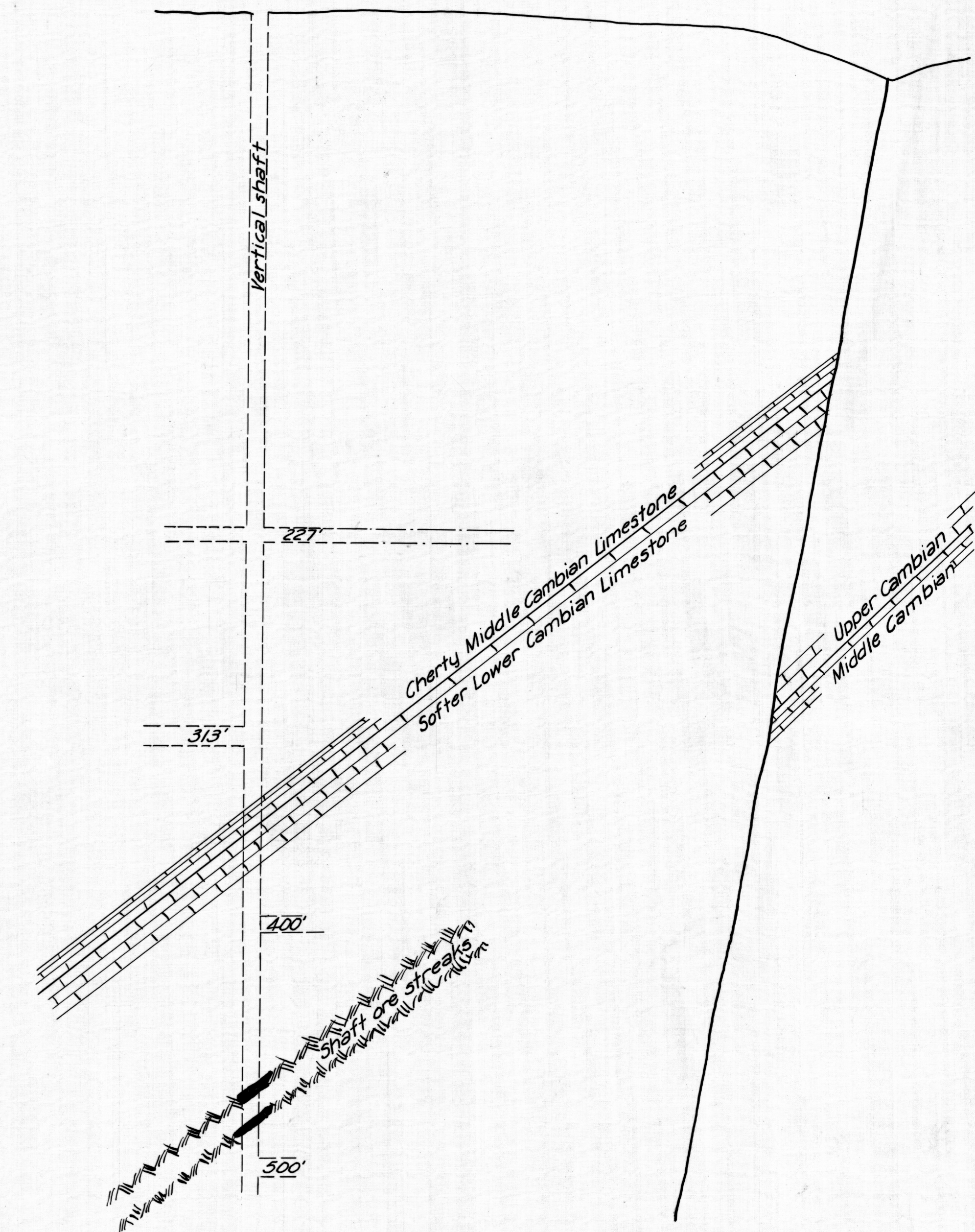
SECTION ON E-E'
