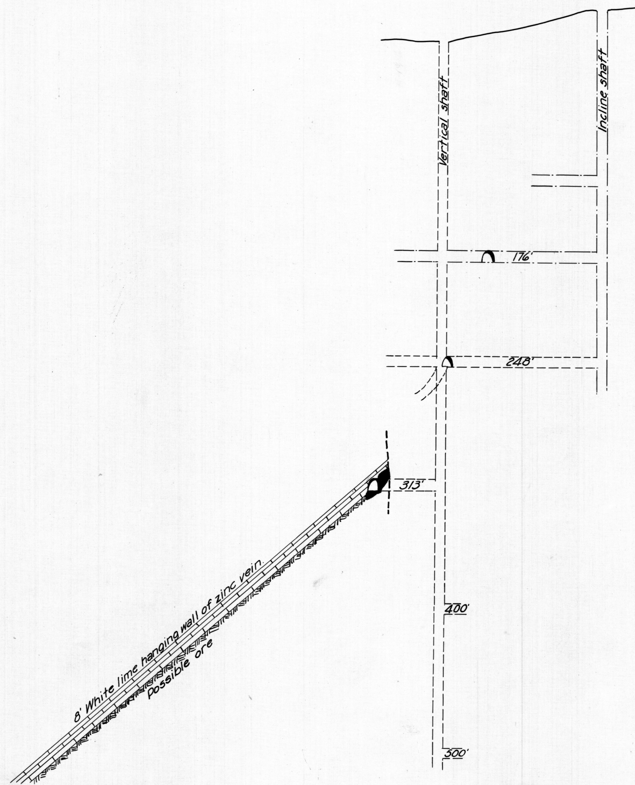
SECTION ON C-C'
