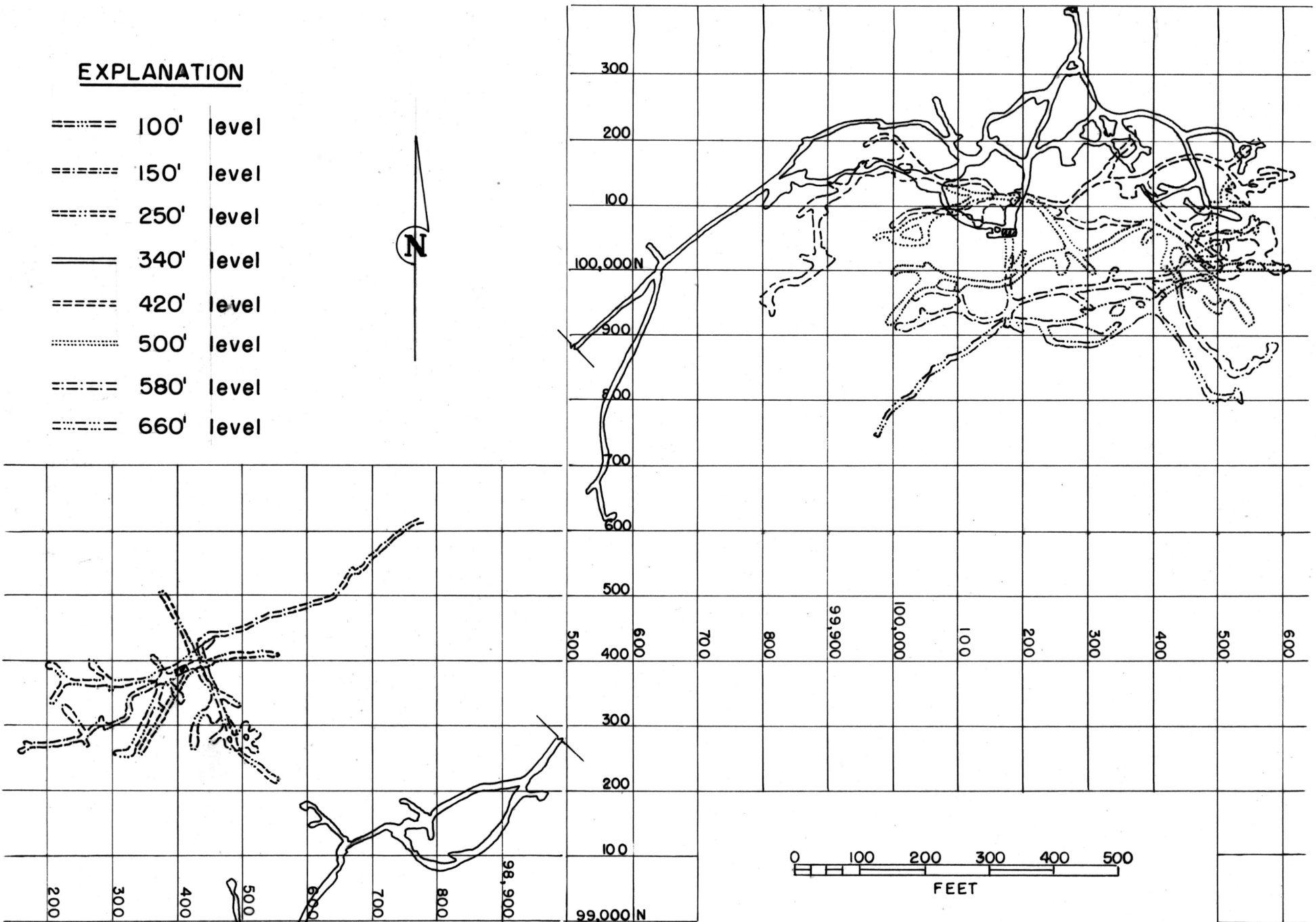
Figure 4.- Plan of workings, San Xavier mine.
