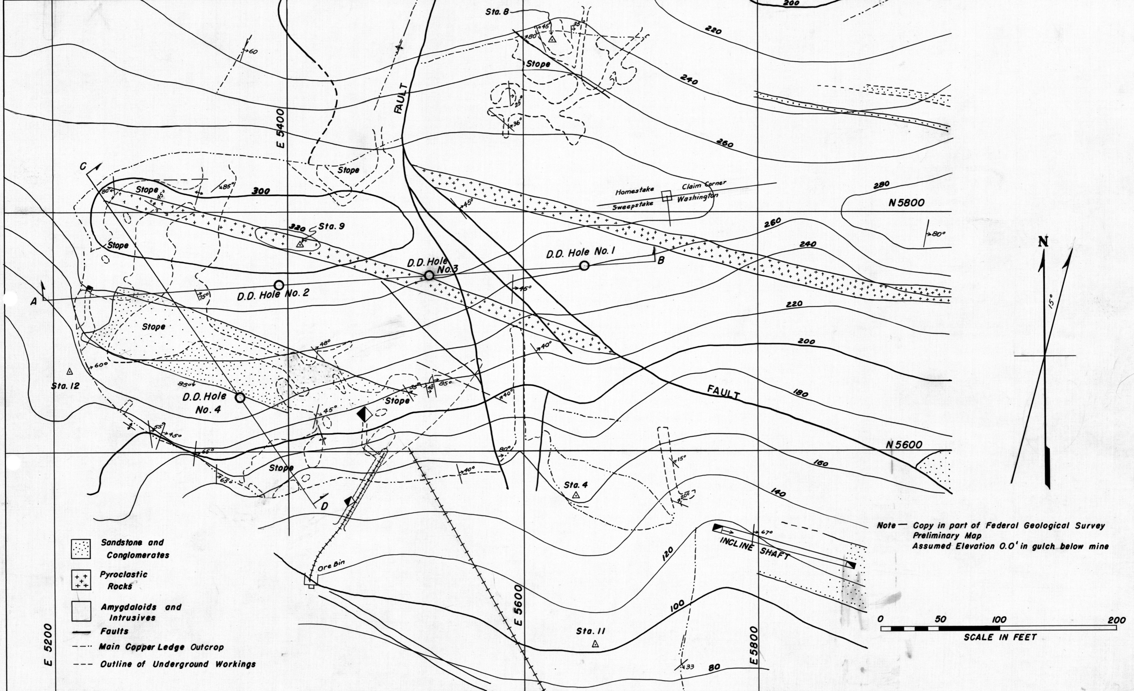
FIG. 3 BULLARD MINE, YAVAPAI COUNTY, ARIZONA
