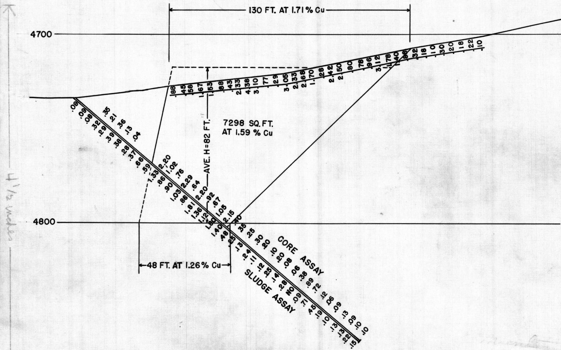
FIG.2.- CROSS-SECTION 748-S, ON CUPRITE CLAIM, ZONIA GROUP
