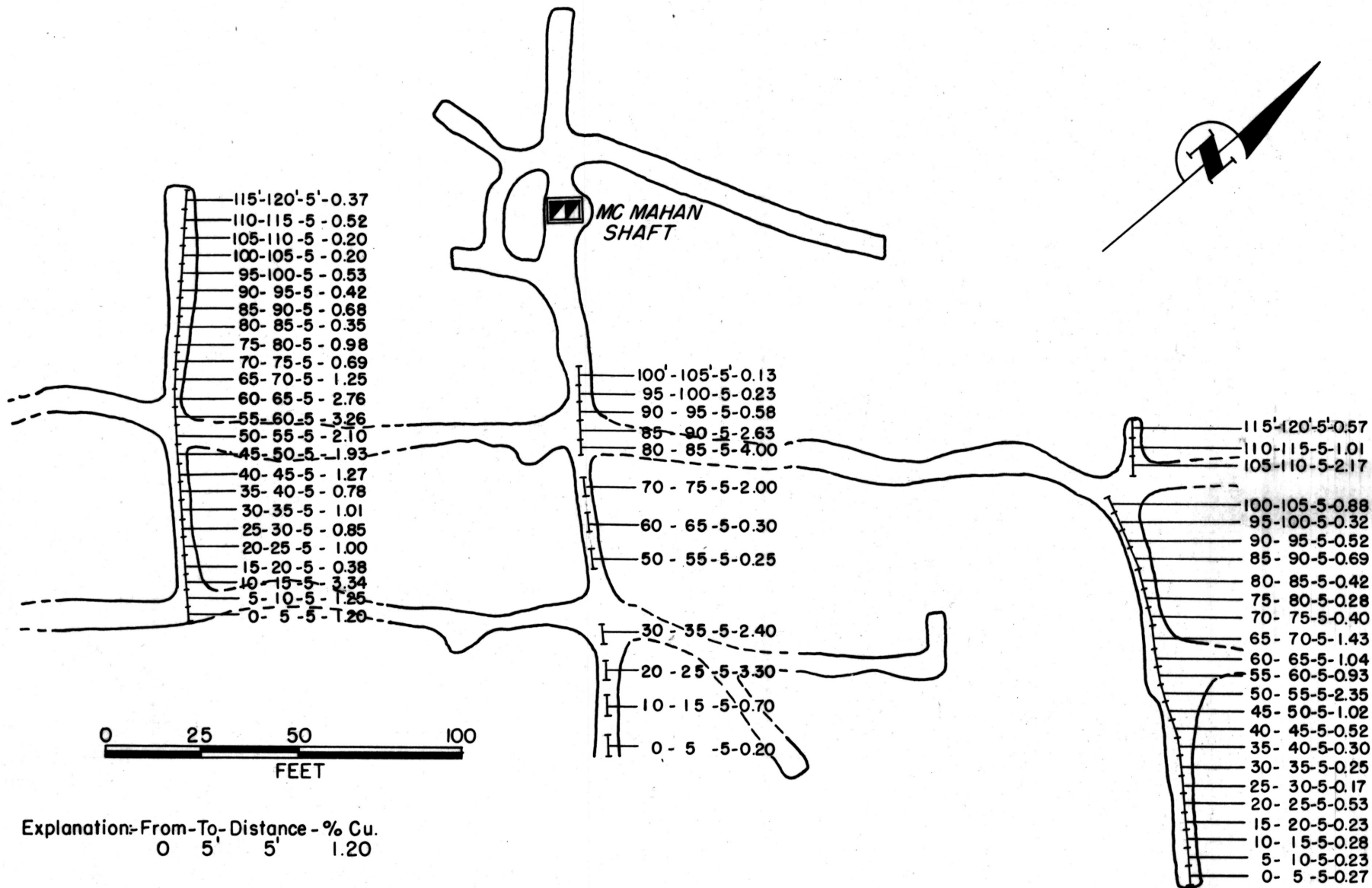
FIG.4- UNDERGROUND CHECK-SAMPLES, ZONIA MINE, PROJ.1417, YAVAPAI CO., ARIZONA
