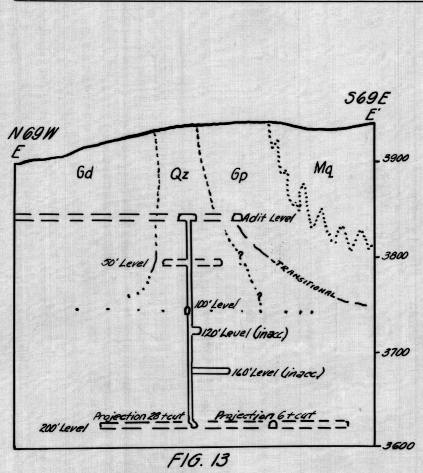
SECTIONS A-A', B-B', C-C', D-D', & E-E' - NEW YEARS EVE MINE
