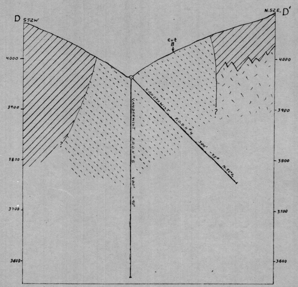
Section D-D'
