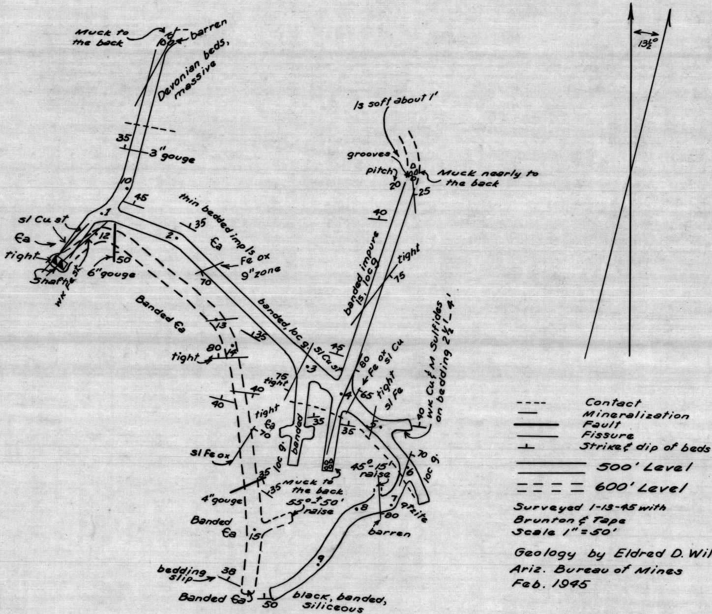
500 & 600' LEVELS OFF THE VERTICAL HAGERMAN SHAFT (Said to be below the collar 487' & 565' respectively)
