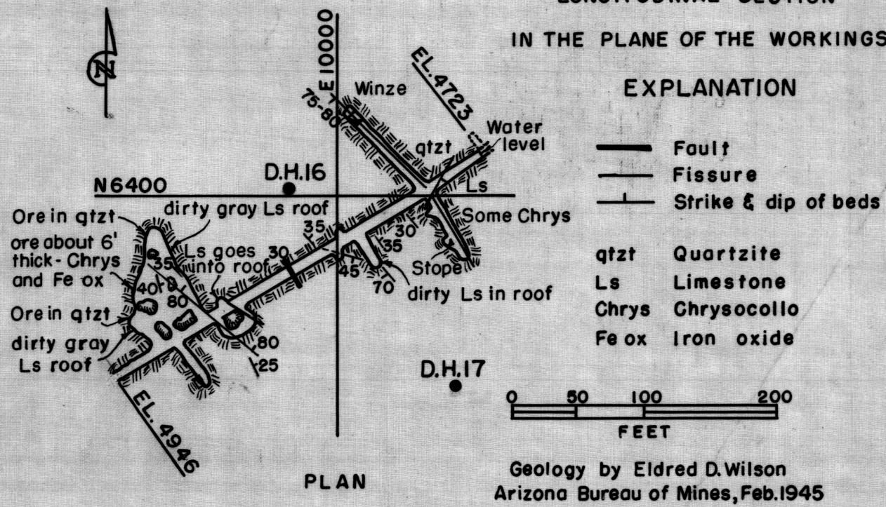
Figure 6.- Plan and sections of O.K. shaft and workings.
