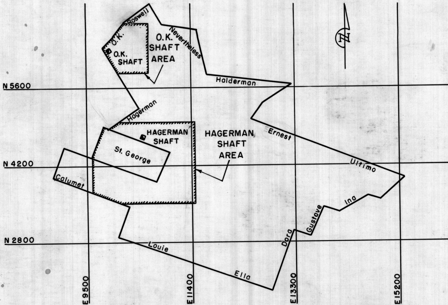
Figure 2.- Property map, Keystone & St. George copper-zinc deposits, Cochise County, Arizona.
