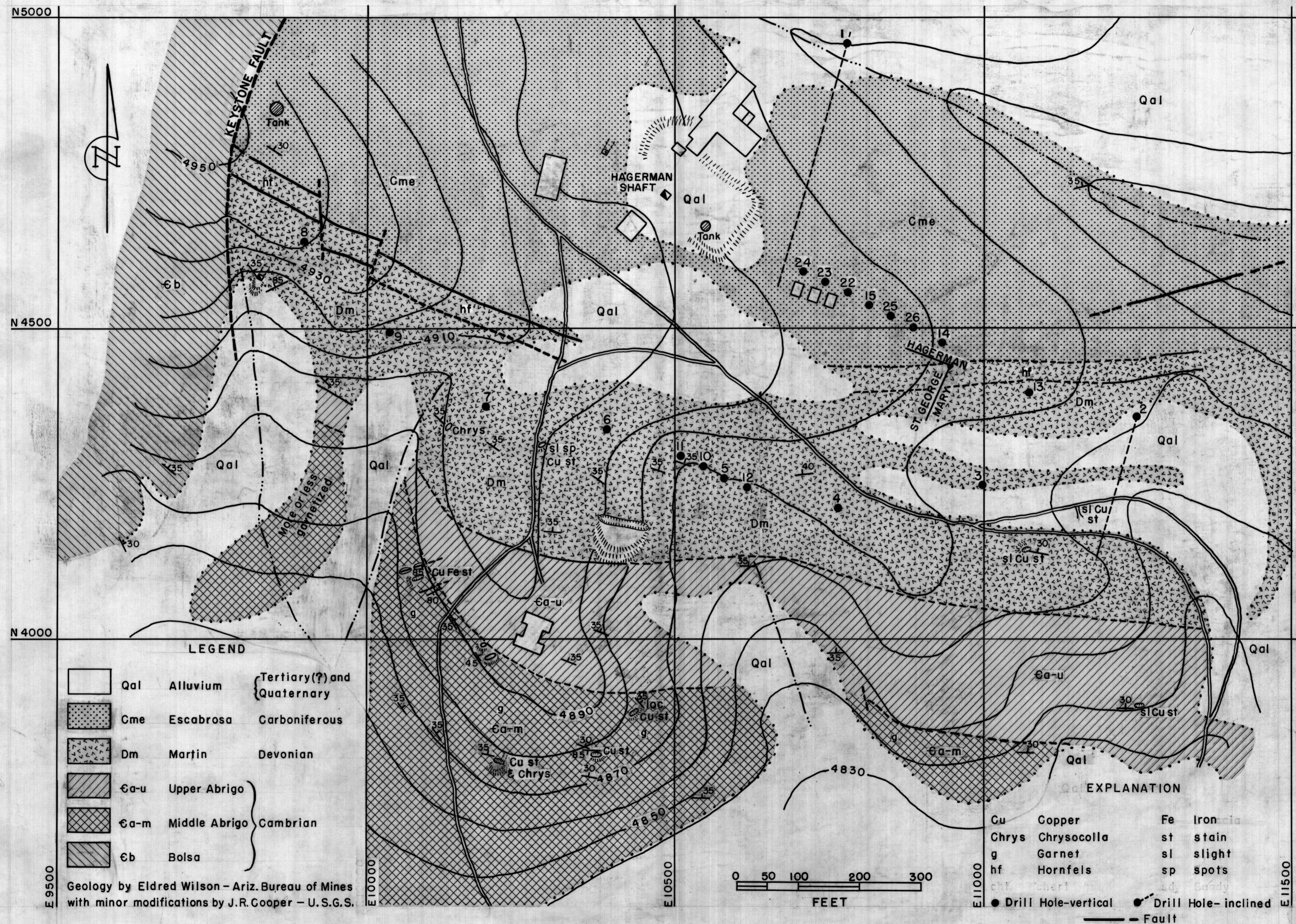
Figure 3.- Geologic map of Hagerman shaft area.
