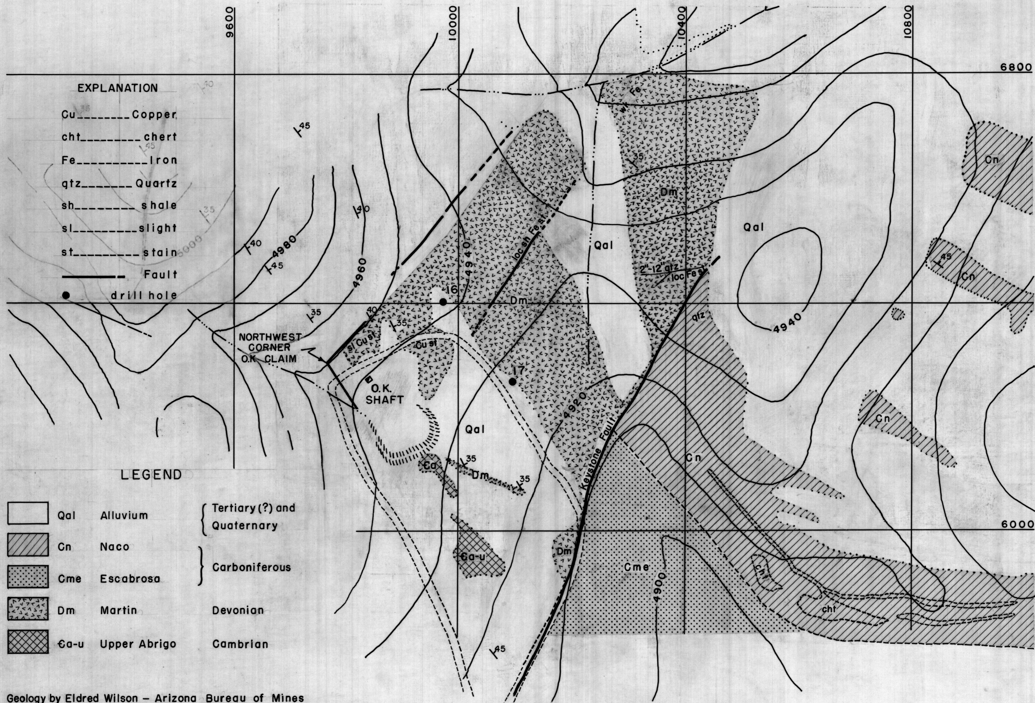
Figure 4.- Geologic map of O.K. shaft area.
