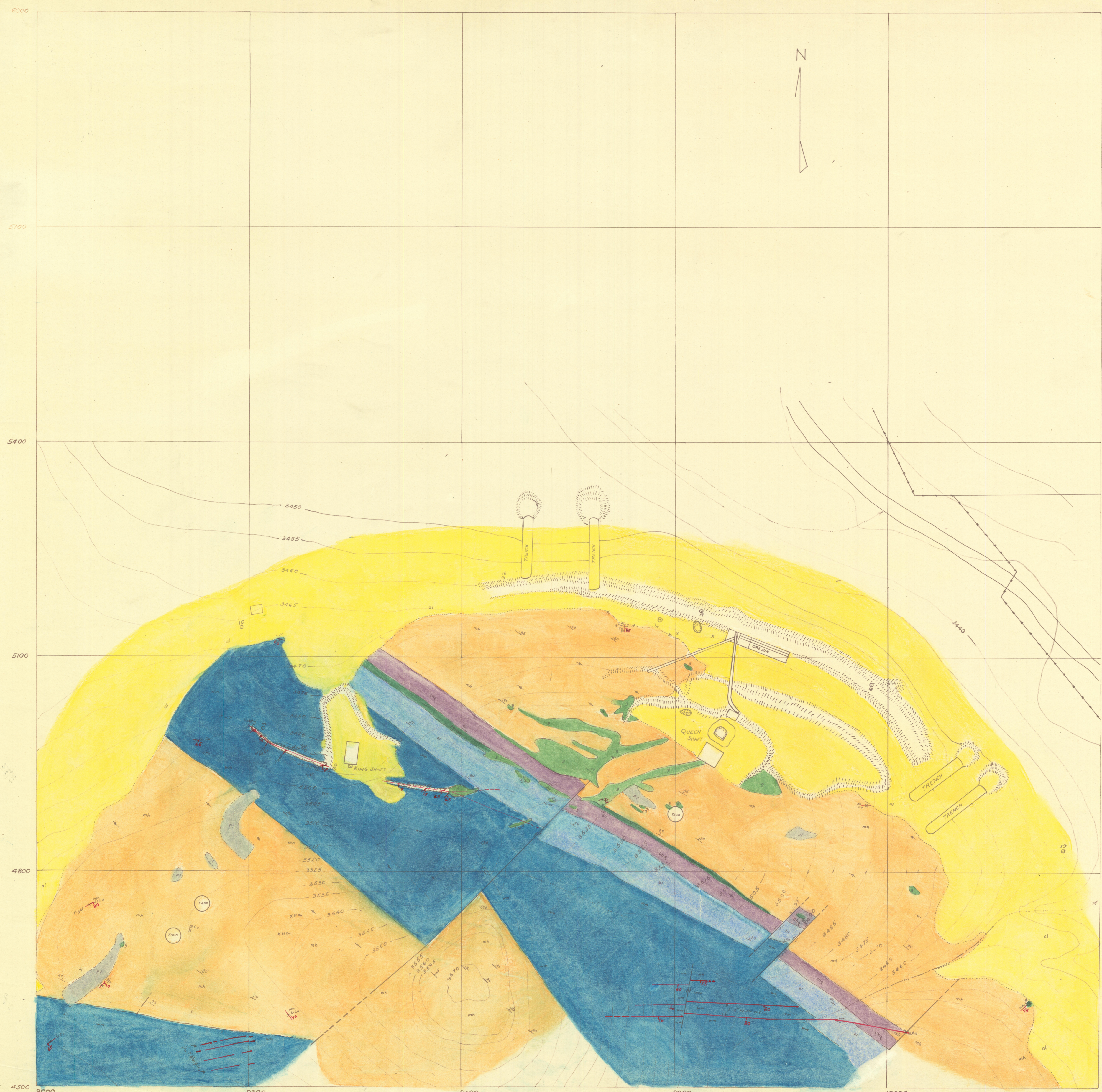
SHEET G-4 TWIN BUTTES COPPER SCALE 1"=50'
