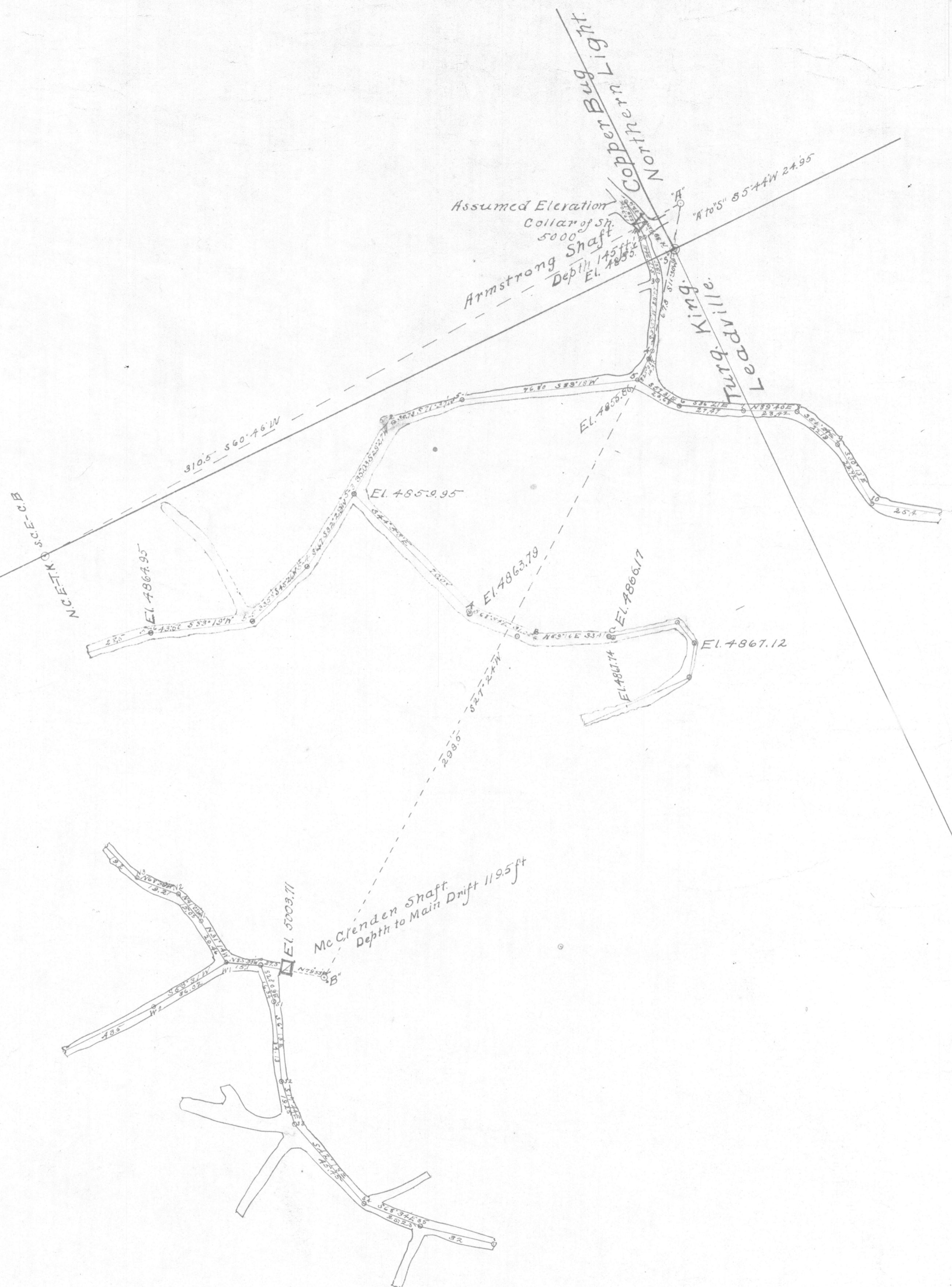
PART OF UNDERGROUND WORKINGS OF THE LEADVILLE MINES. Surveyed by J.A. Rockfellow January 26-31 1925 Scale 1 inch 30 feet.
