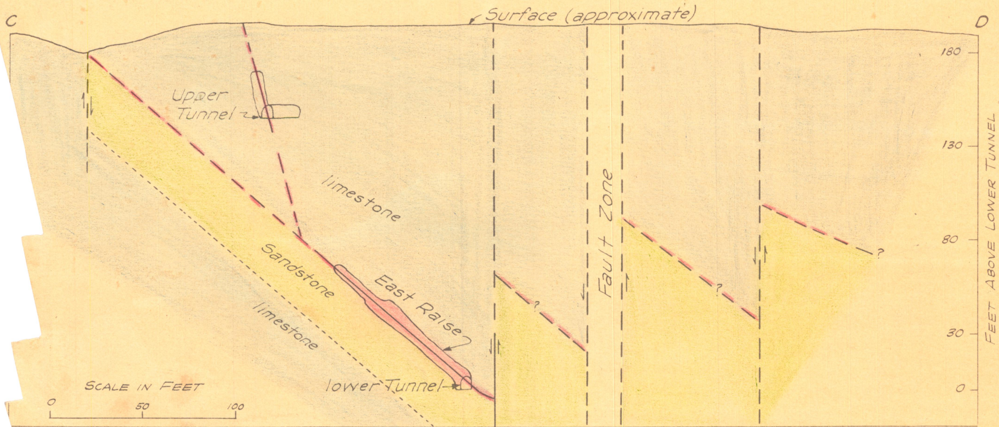
Figure 2-b. VERTICAL SECTION ALONG LINE C-D OF { Figure 2 Plate II
