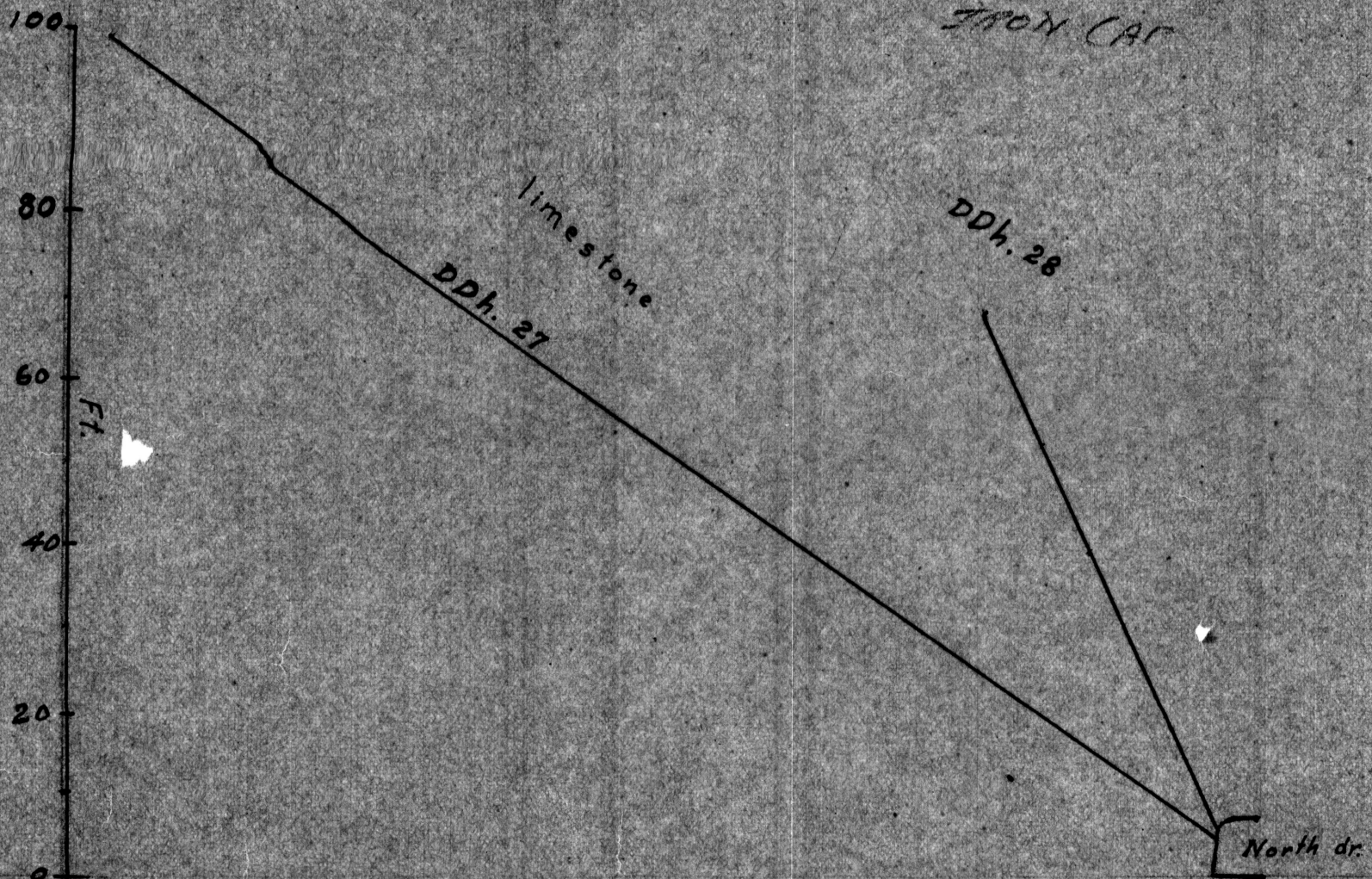
PLATE D-7 SECTION ALONG HOLES 27, 28
