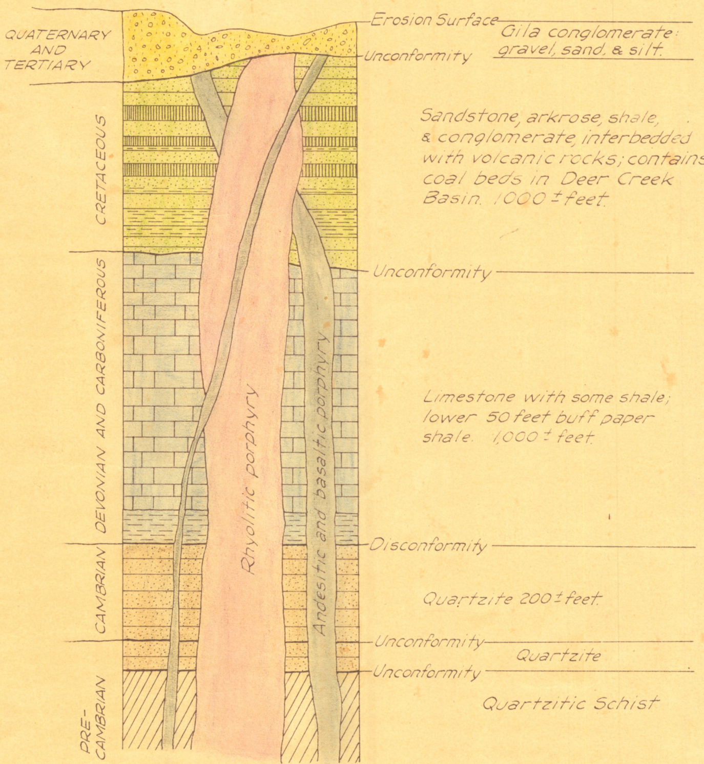
Figure 1 GENERALIZED COLUMNAR SECTION
